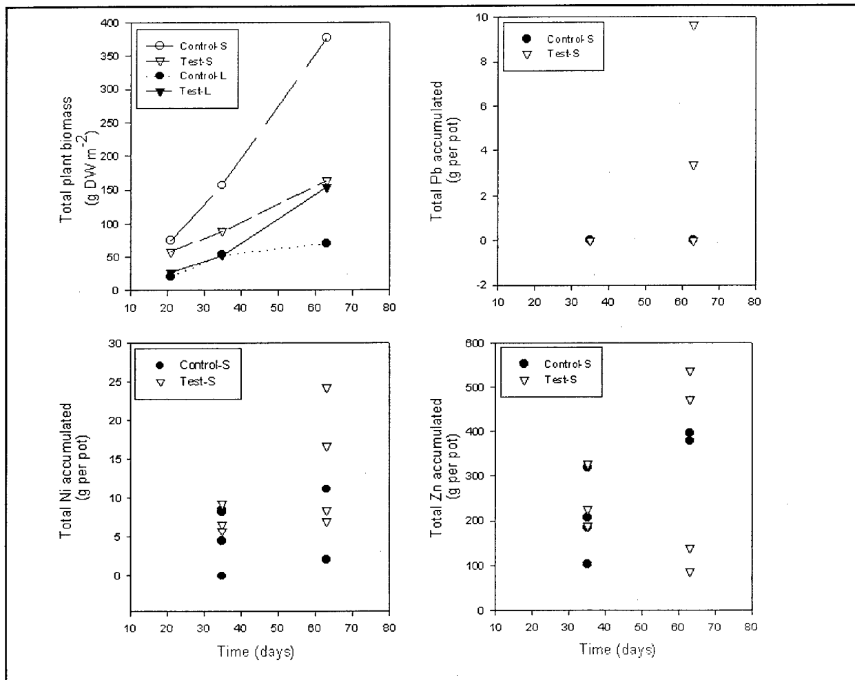
Figure 2. Average growth response ( N = 4 ) of C. esculentus plants cultivated on test dredged material and control soil in 2-L pots, with a small (S, 0.0167 m 2 ) and large (L, 0.0238 m 2 ) surface area (top left). Bioaccumulation of lead, nickel, and zinc was also measured; of the bioaccumulation data, only those pertaining to pots with a small surface area are shown
