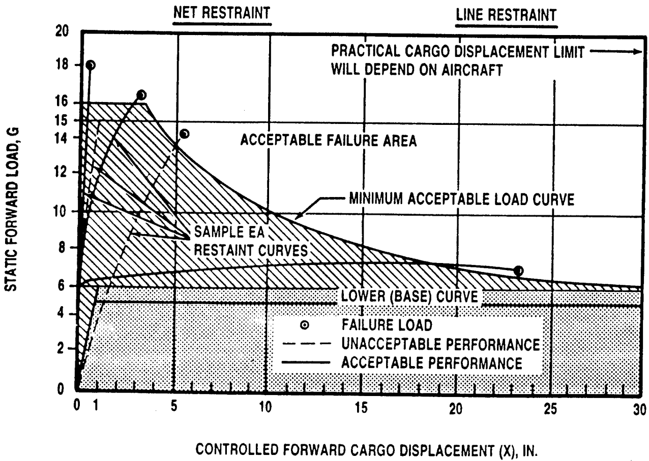
FIGURE 9. Forward load - displacement for energy-absorbing cargo restraint.
