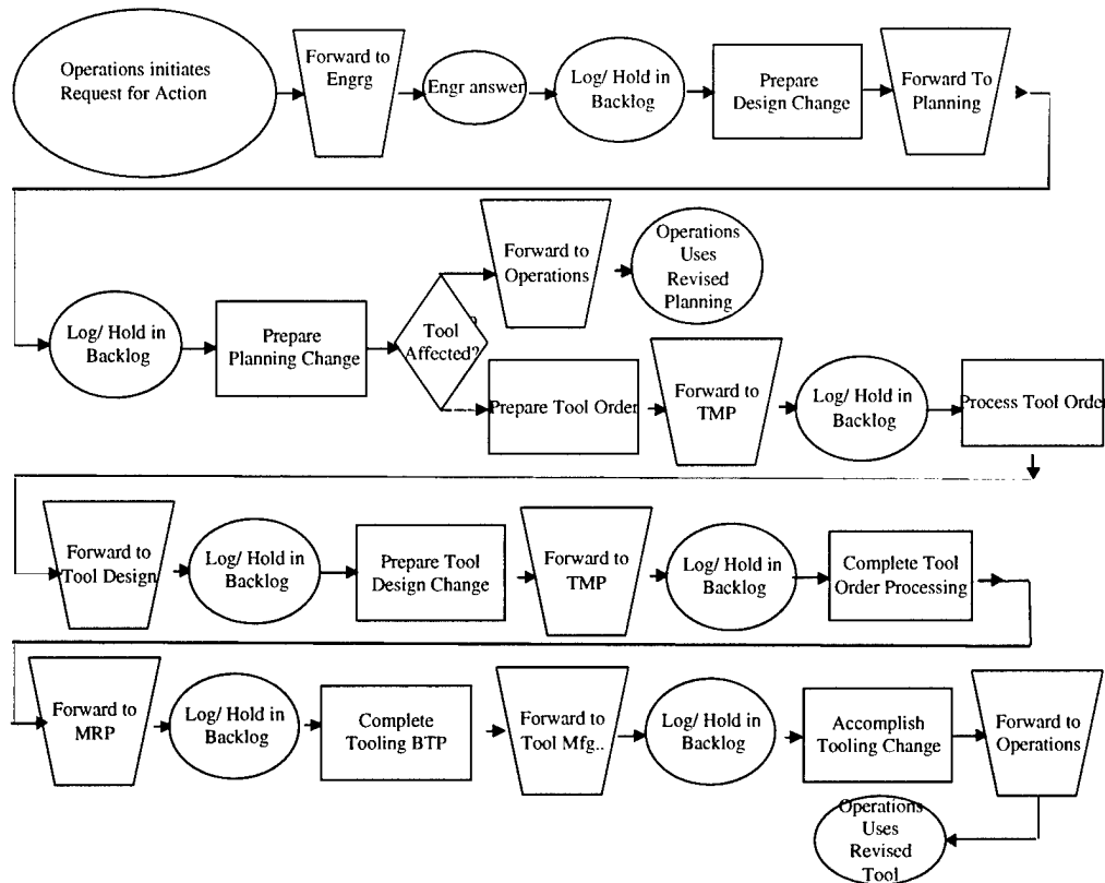
Figure 13. F-16 BTP Pre-improvement VSM [43]
