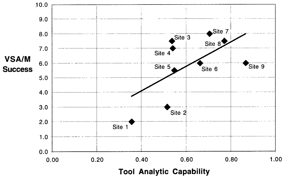
Figure 23. Success-Capability Correlation
