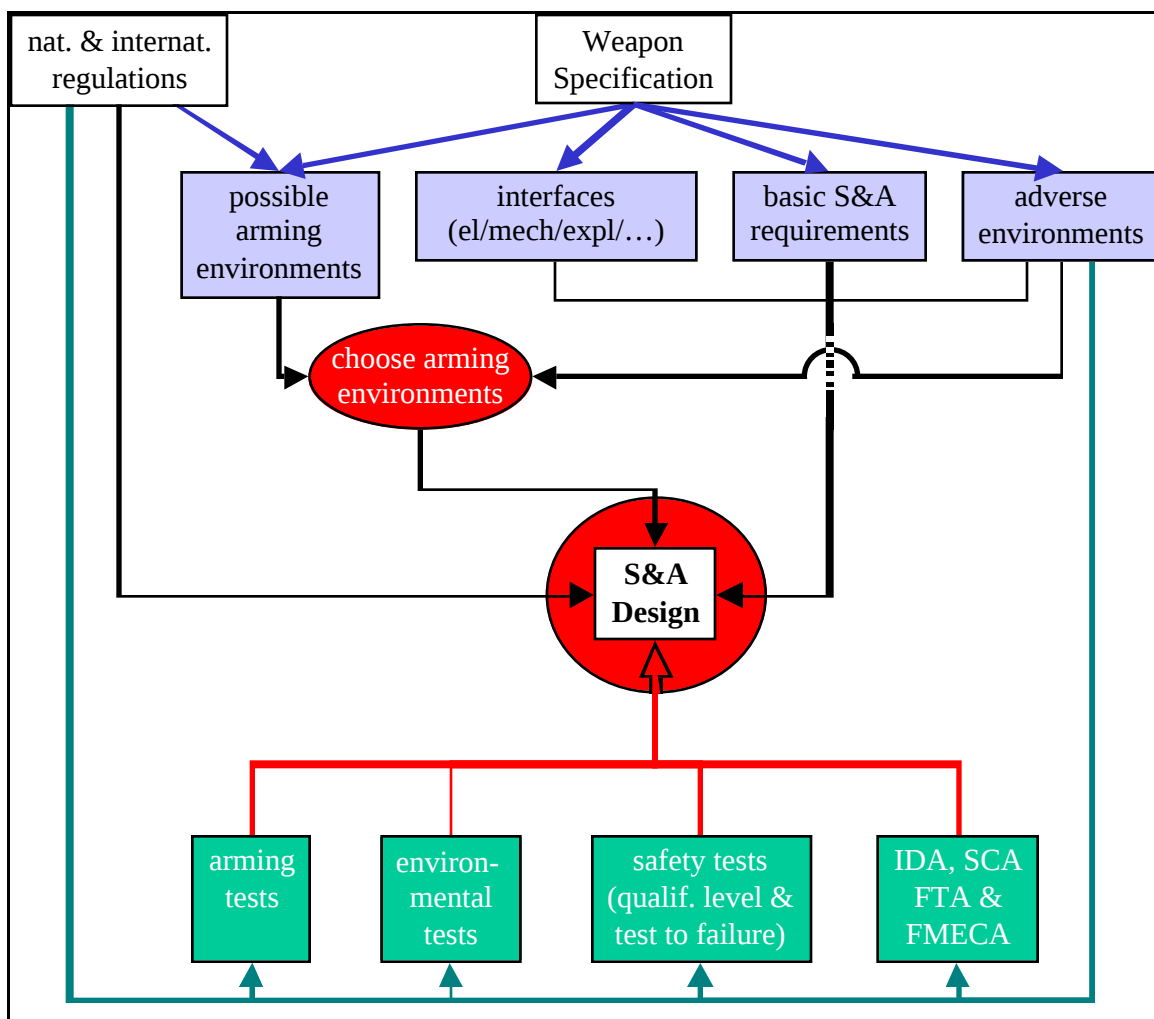
FIGURE 6. Weapon Specification and Requirements (the Starting Points for Every S&A Device Design).
