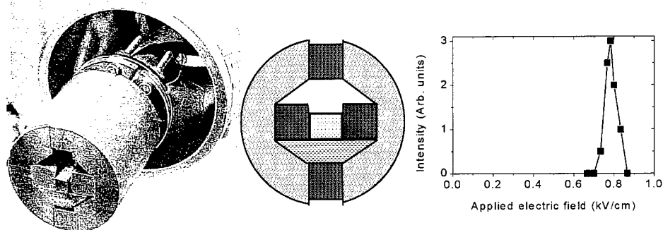
Figure 1. (Left) Photograph of permanent magnets, soft-iron yoke, copper cold finger and p-Ge crystal attached to a 10 K 0.5 W closed cycle refrigerator. (Middle) Schematic of permanent magnets (dark squares), laser crystal (light square), Fe yoke (parentheses) and Cu cold finger (trapezoid). The diameter of the magnet-yoke system is 1.5 inch. (Right) Demonstration of laser action, using permanent magnet assembly in liquid helium.
