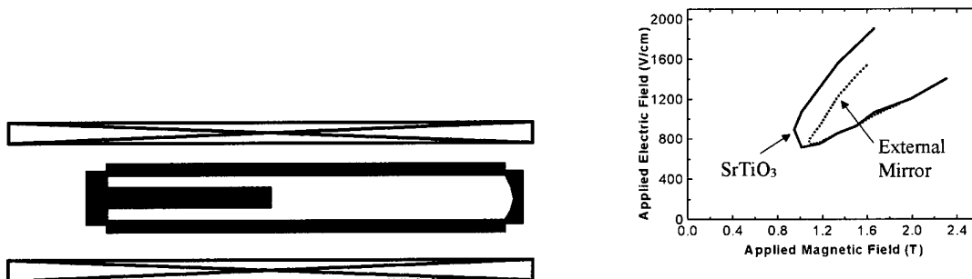
Figure 4 (Left). Schematic of external cavity p-Ge laser, without tuning elements. (Right) Laser generation regions for external cavity and also for traditional cavity with SrTiO 3 mirrors.
