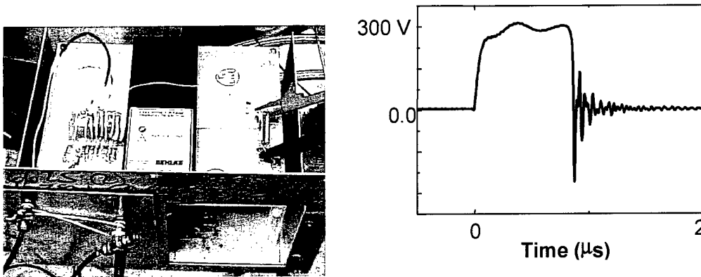
Figure 6. Photograph of the MOSFET pulser. Pulse shape for a resistive load.
