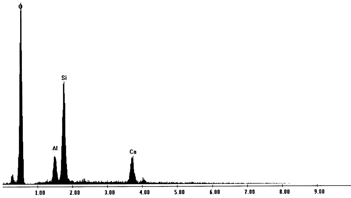
Figure 15. EDX spectrum of fibers from thrust chamber glass fabric overwrap.
