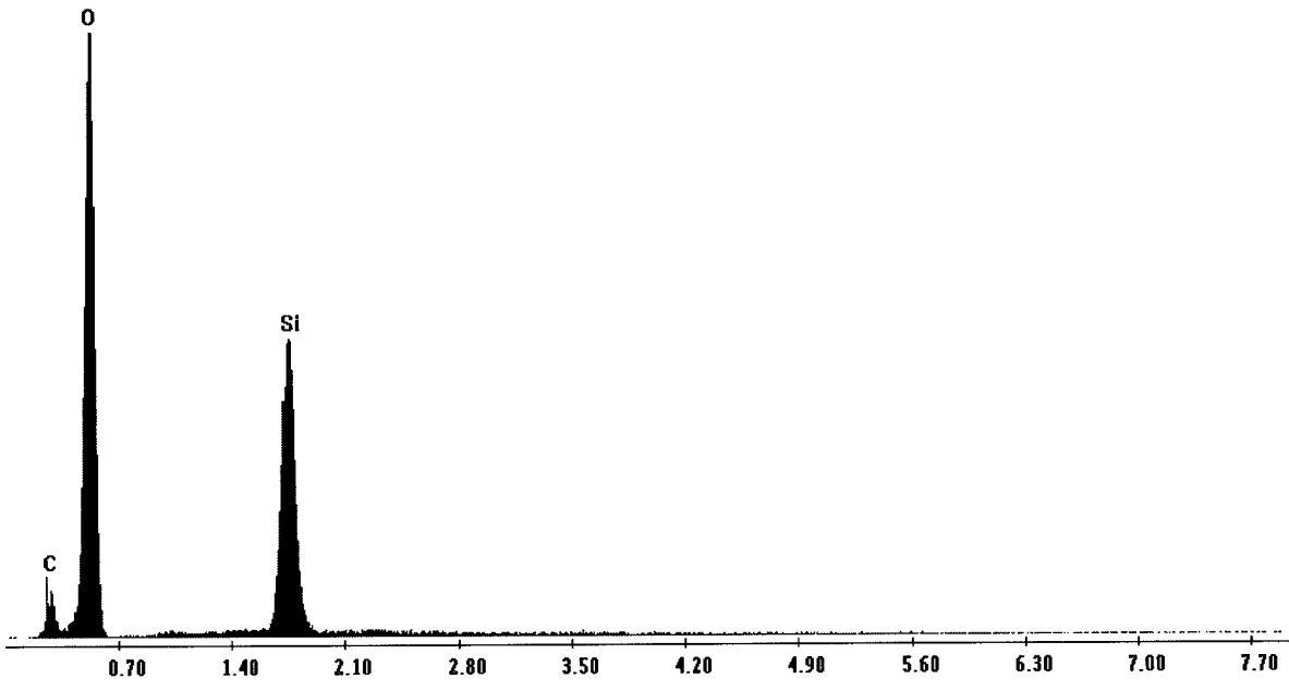
Figure 14. EDX spectrum of fibers from silica phenolic liner.
