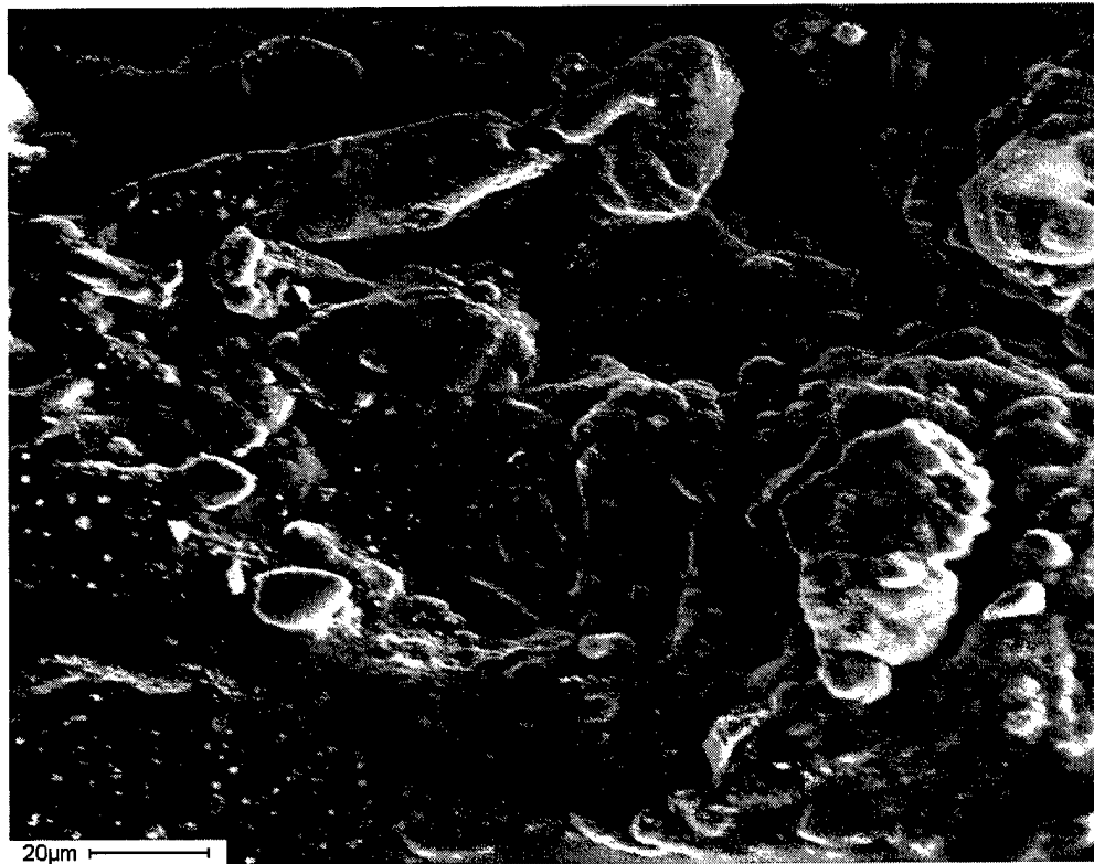
Figure 9. SEM photographs of metallic deposits on debris.
