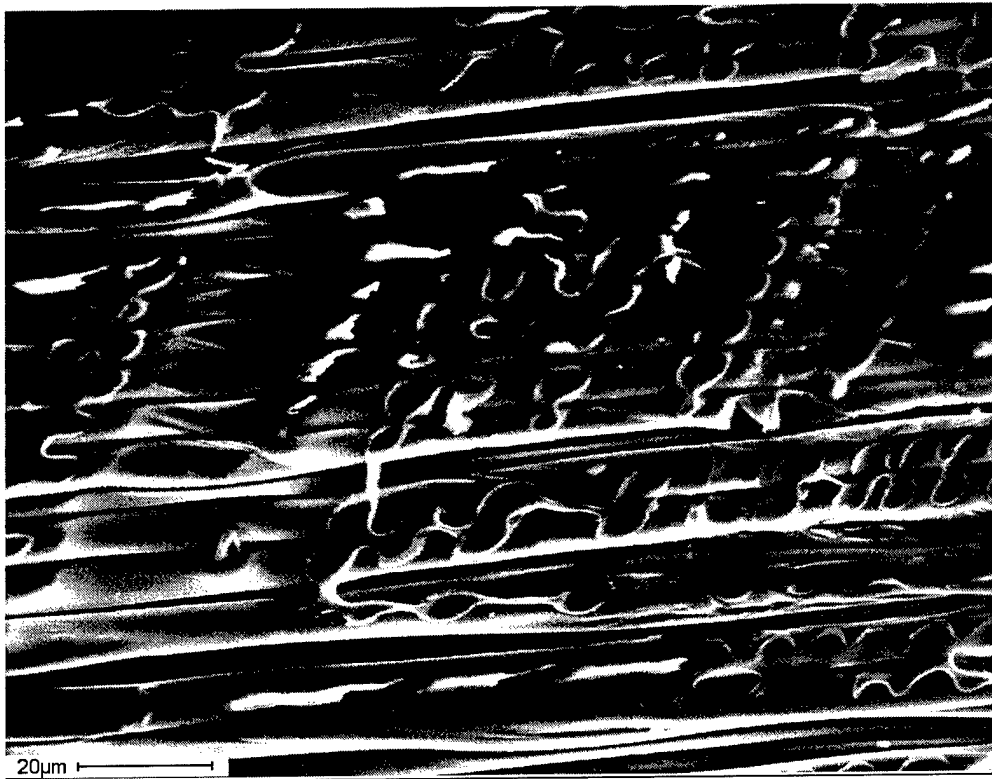
Figure 6. SEM photographs of fibers in the debris.
