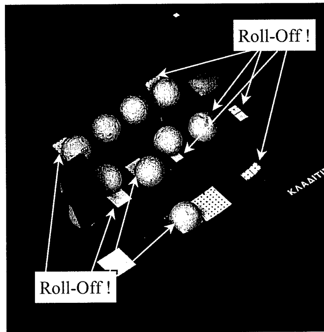
Figure 4-19: SEM showing an extreme example of roll-off due to contamination.
