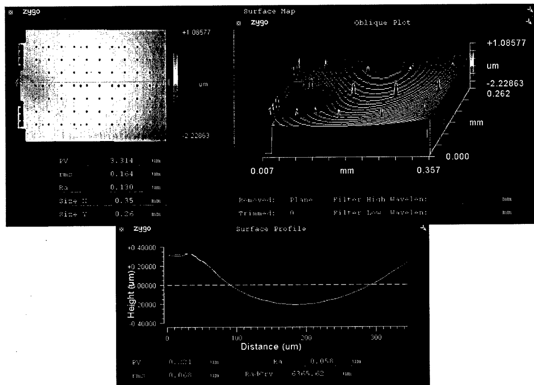
Figure 6-7: Output of the Zygo interferometric microscope showing the measurement of radius of curvature of solder on poly2.
