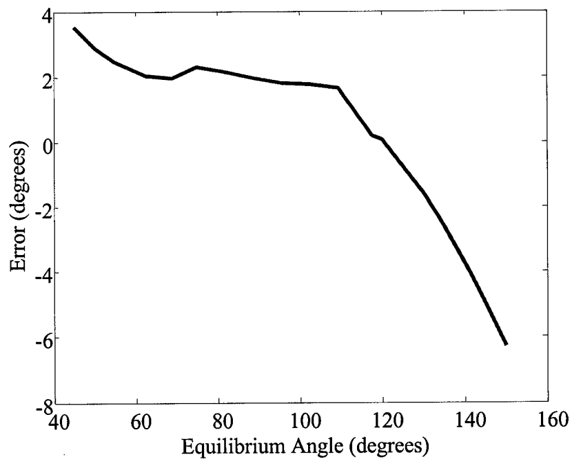
Figure 5-8: Plot of error between geometric model equilibrium angle predictions and Surface Evolver predictions for different square solder pad lengths while keeping a fixed volume of solder equivalent to an 8 mil diameter sphere.
