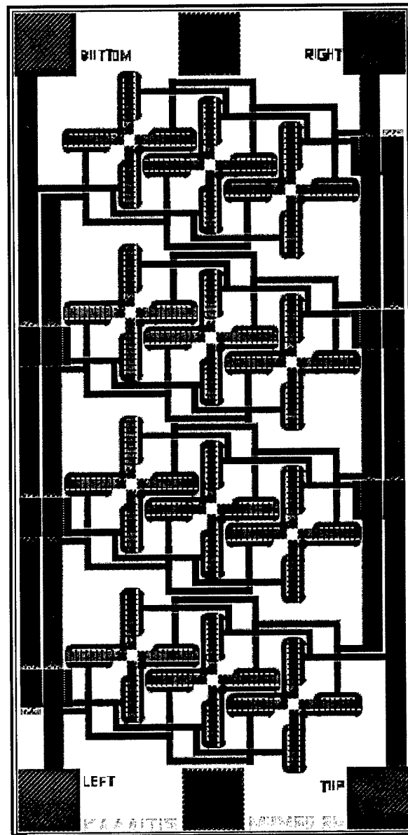
Figure E-21: MUMPs 36 Die 1; 4 mm \times 2 mm; 2-D micro conveyor with gold on polysilicon thermally actuated bilayer cantilevers as conveyer arms.
