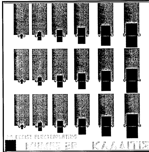
Figure E-31: MUMPs 38 Die 3; 2 mm × 2 mm; solder self-assembled simple plates where the solder is deposited on the solder pads using mask-less electroplated solder. In the unreleased state, the whole die is covered in PSG except for the solder pads and bond pads.
