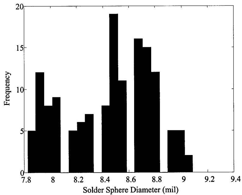
Figure 6-3: Histogram of 8 mil ball measurements.
