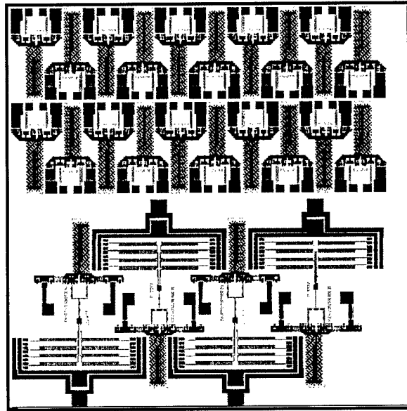
Figure E-1: MUMPs 27; 2 mm \times 2 mm; microrobot leg array for thermally evaporated indium solder self-assembly.
