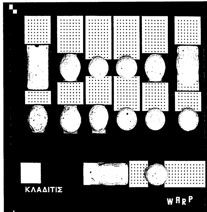
Figure 4-7: SEM of an unreleased, preflowed chip containing an array of 8 mil warp version test structures.
