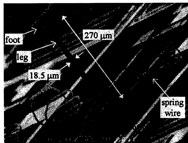
Fig. 4. SEM of an assembled microrobot leg with two degrees-of-freedom motion.
