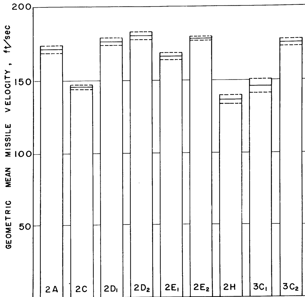
Fig. 5.16—Geometric mean velocities for missiles from various traps. Trap 2H was in an open area 100 ft behind the rambler house at the 4700-ft range; other traps indicated were inside the houses behind windows facing Ground Zero—2A, 2C, 2D 1 , 2D 2 , 2E 1 , and 2E 2 at the 4700-ft range and 3C 1 and 3C 2 at the 5500-ft range. Dashed lines represent the standard error of the mean.
