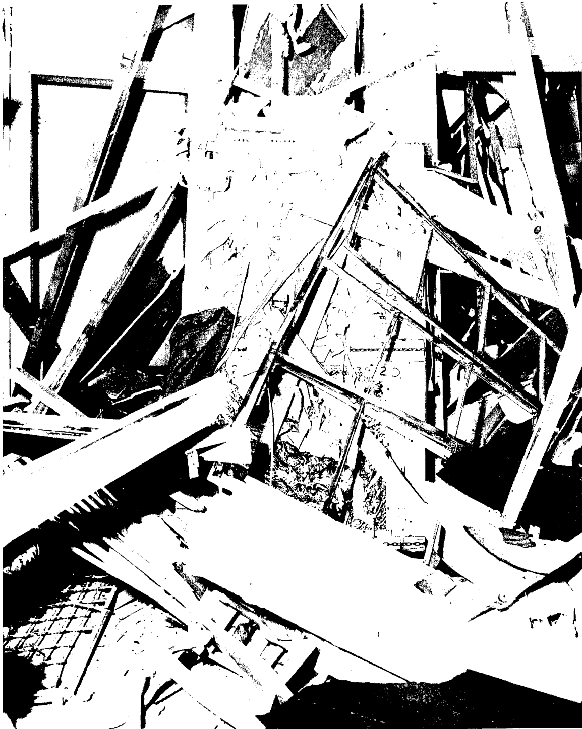
Fig. 4.15—Traps 2D 1 and 2D 2 after the detonation. See Fig. 4.14.
