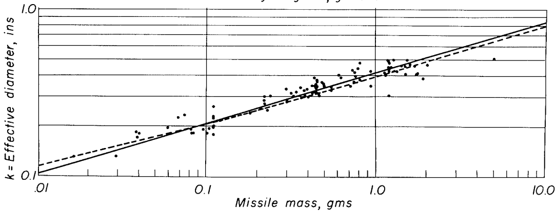
Fig. 3.3—Effective diameter of glass-fragment missiles as a function of missile mass for penetration into Styrofoam 22.
