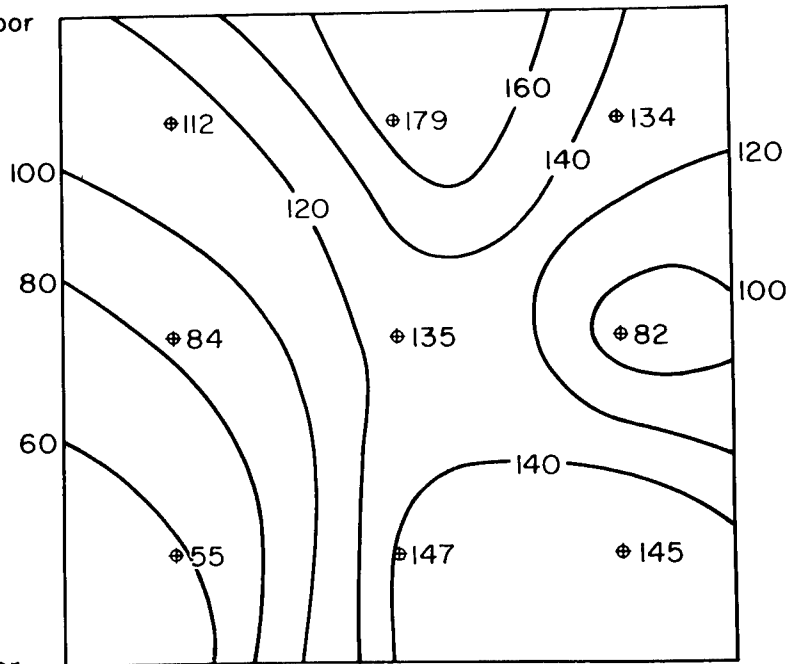
Fig. 5.30—Spatial distribution of missiles passing through the front surface of traps 2A and 2C. Numbers indicate missiles per square foot.
