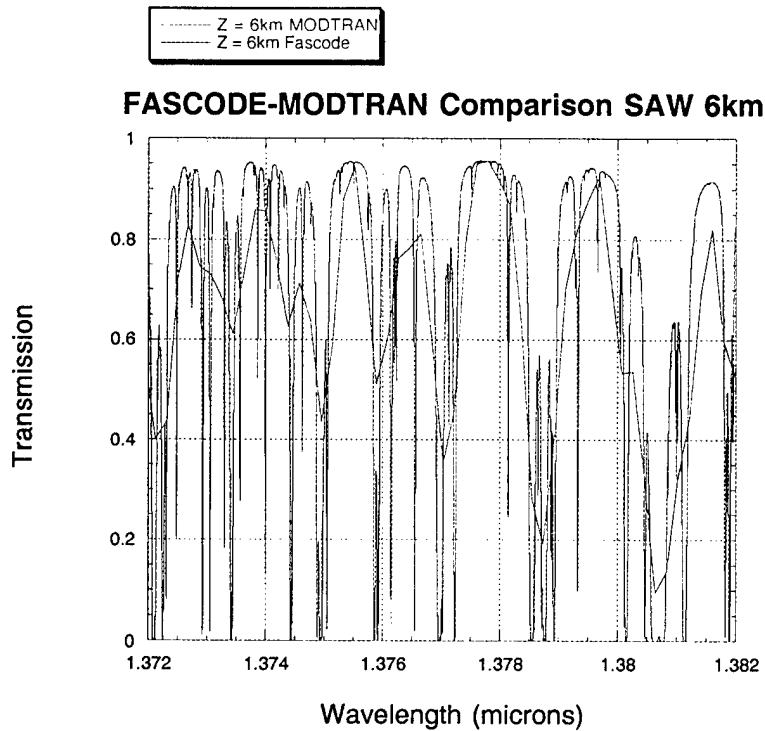
Figure 4. Comparison of the calculated transmission from FASCODE and MODTRAN for the 1.372–1.382 \mu\text{m} band for the Mid-Latitude-Summer (MLS) and Sub-Arctic-Winter (SAW) atmosphere models for a 6-km cloud height.
