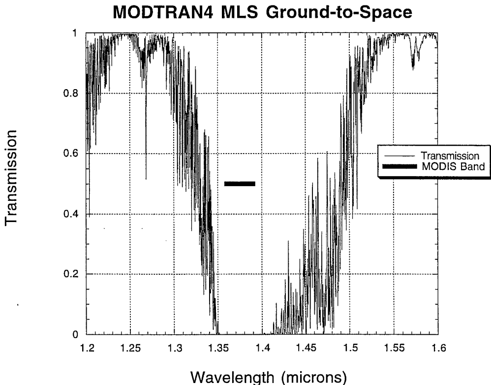
Figure 1. MODTRAN atmospheric transmission from space to sea level for a mid-latitude summer model atmosphere in the vicinity of the 1.375 \mu\text{m} water-vapor absorption band. The central part of the band is virtually opaque. Also shown is the position of the nominal MODIS band.
