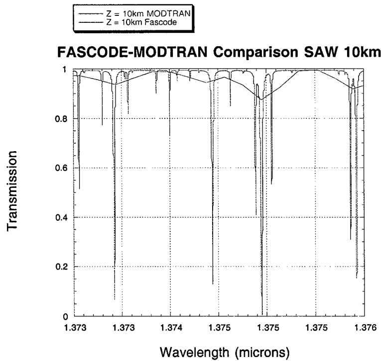
Figure 7. Comparison of the calculated transmission from FASCODE and MODTRAN for the 1.373–1.376 \mu\text{m} band for the Mid-Latitude-Summer (MLS) and Sub-Arctic-Winter (SAW) atmosphere models for a 10-km cloud height.
