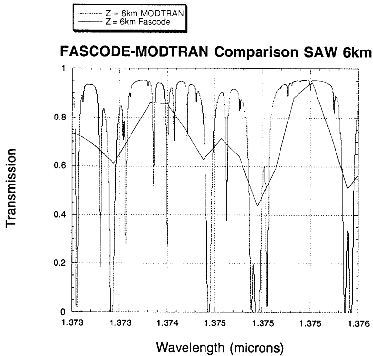
Figure 6. Comparison of the calculated transmission from FASCODE and MODTRAN for the 1.373–1.376 \mu\text{m} band for the Mid-Latitude-Summer (MLS) and Sub-Arctic-Winter (SAW) atmosphere models for a 6-km cloud height.
