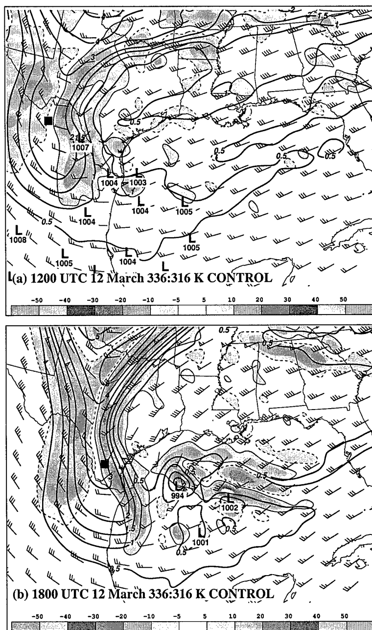
Figure 4.51: CONTROL IPV analysis in the column from 336 K to 316 K, with IPV contoured at 0.5 PVU and every 1.0 PVU thereafter, IPV advection ( -\mathbf{V} \bullet \nabla IPV ) shaded at 5 PVU day -1 and every 10 PVU day -1 thereafter (negative dashed contour outline), and layer-averaged wind vectors (in m s -1 ). Valid (a) 1200 UTC 12 March, (b) 1800 UTC 12 March, (c) 0000 UTC 13 March, and (d) 0600 UTC 13 March.
