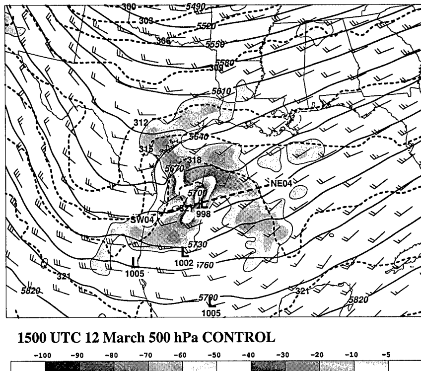
Figure 4.11: CONTROL 500 hPa fields at 1500 UTC 12 March. Depicted are geopotential height (contoured every 30 m), isentropes (contoured every 3 K), standard wind vectors (in \text{m s}^{-1} ), and vertical velocity (shaded in \mu\text{bar s}^{-1} ). Surface low pressure centers are indicated.
