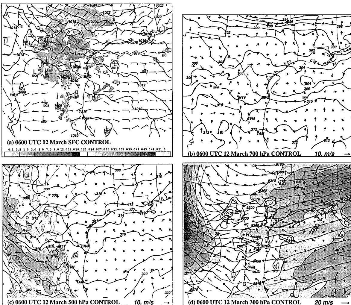
Figure 3.9: As in Fig. 3.5, except for 0600 UTC 12 March.
