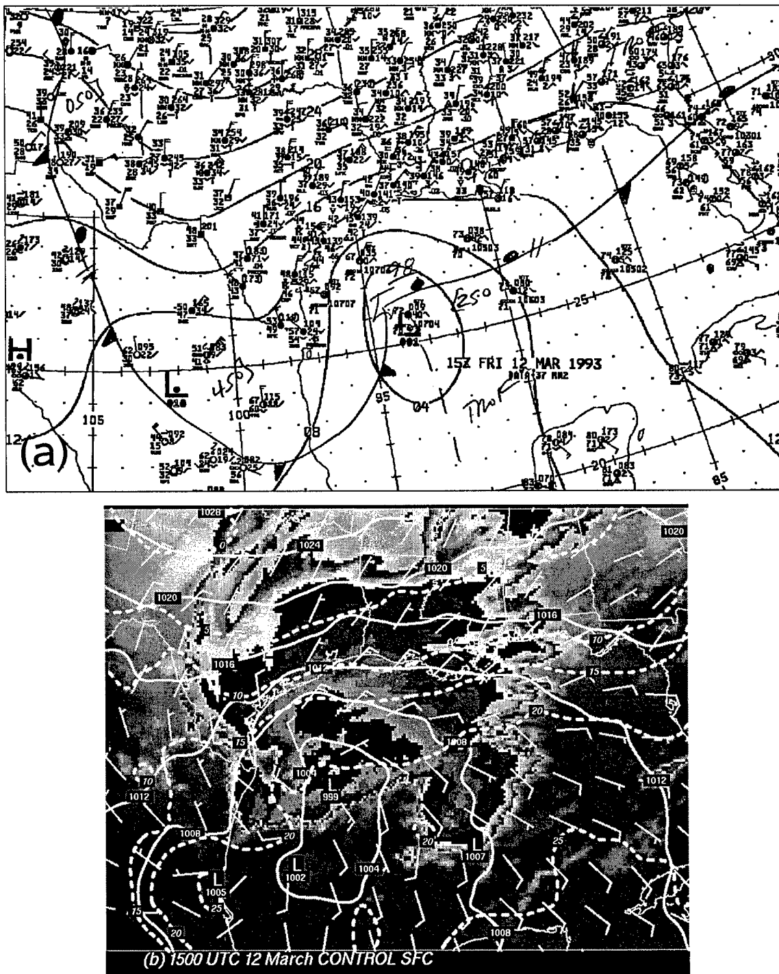
Figure 4.5: Observed and simulated surface fields at 1500 UTC 12 March. (a) NCEP surface analysis and (b) CONTROL surface fields on GOES-7 IR imagery, depicting PMSL (solid every 4 hPa), surface temperature (dashed every 5 C), and total wind vectors (in \text{m s}^{-1} ).
