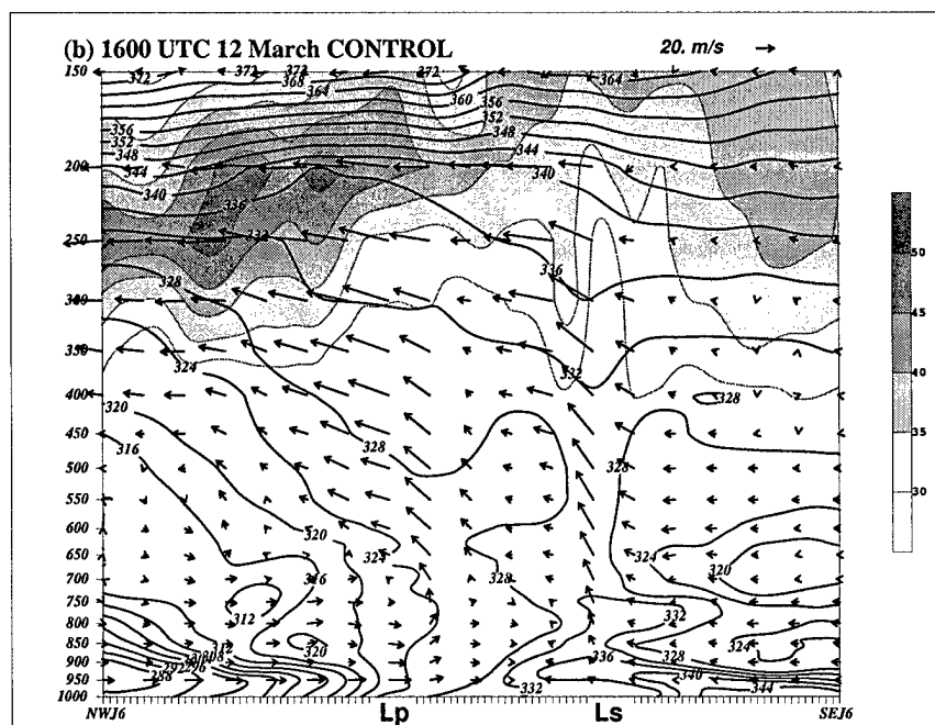
Figure 4.27: CONTROL jet structure at 1600 UTC 12 March, depicting (a) 250 hPa ageostrophic wind vectors (reference vector in lower right of panel), divergence (contoured every 1 \times 10^{-4} ), and total isotachs (shaded > 35 \text{ m s}^{-1} ); and (b) cross-section through the PFJ and STJ entrance regions; ageostrophic circulation vectors, isotachs (shaded > 35 \text{ m s}^{-1} ), and equivalent potential temperature (contoured every 4 K). Plane of the cross-section is indicated in (a). Positions of the primary (Lp) and secondary (Ls) low are indicated relative to the plane of the cross-section.
