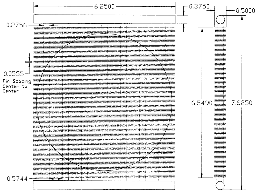
Figure 1: Drawing of Fin-tube Heat Exchanger (dimensions in inches)
