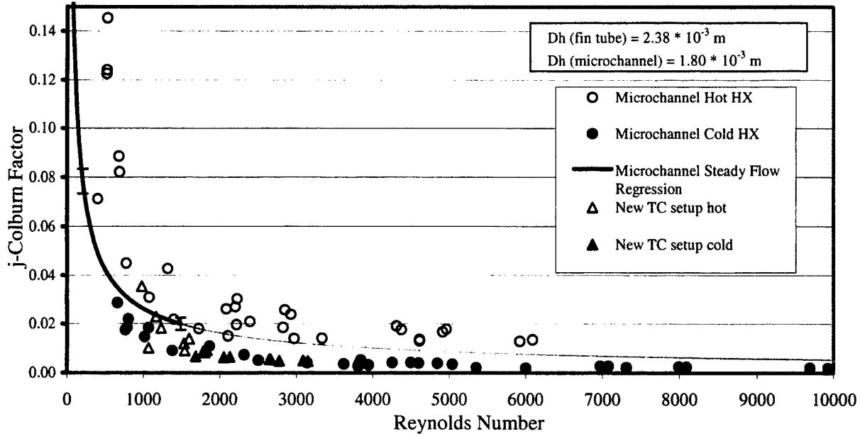
Figure 16. j-Colburn vs. Acoustic Reynolds Number; Microchannel Heat Exchanger, Computed from Radial Thermocouple Array Data ;Dotted line denotes the extrapolation of the experimental data
