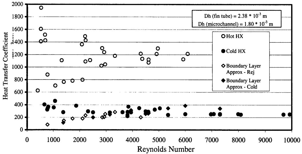
Figure 14. Heat Transfer Coefficient (W/m 2 ·K) vs. Acoustic Reynolds Number for Periodic Flow; Microchannel
