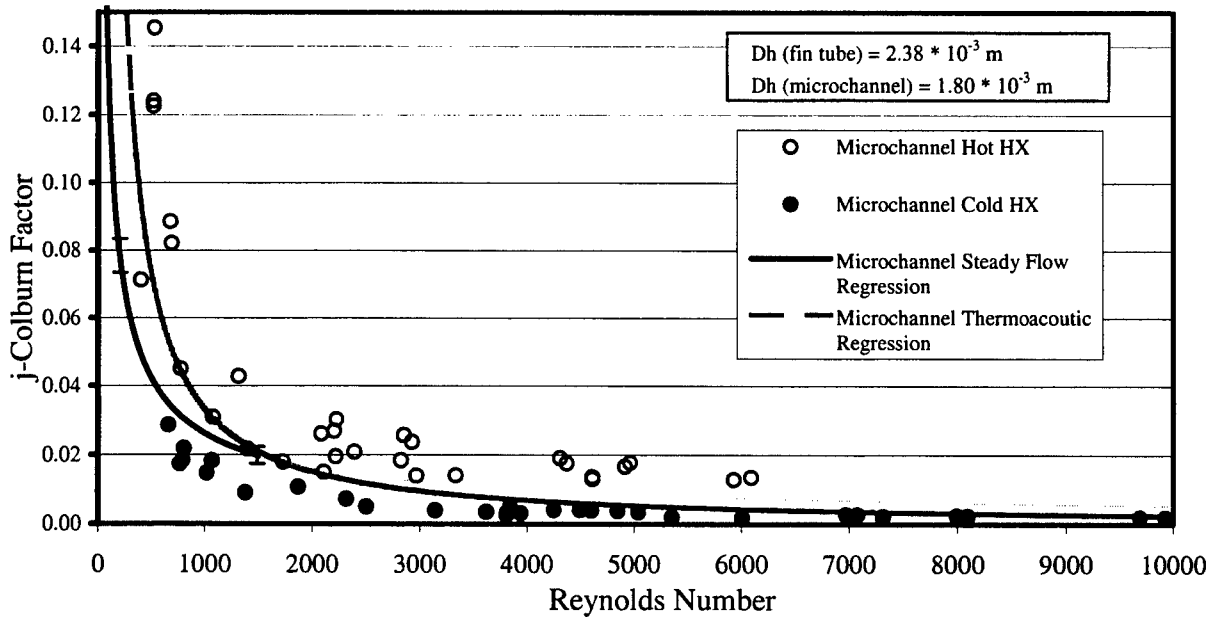
Figure 15. j-Colburn vs. Acoustic Reynolds Number Regression; Microchannel Heat Exchanger ;Dotted line denotes the extrapolation of the experimental data
