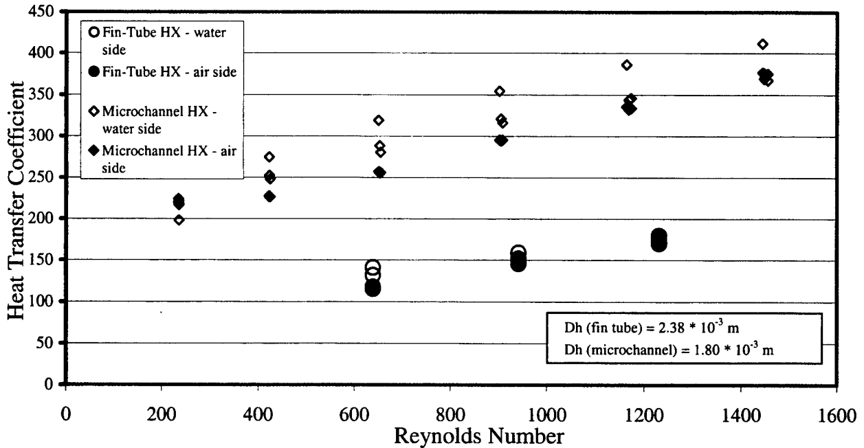
Figure 10. Steady Flow Heat Transfer Coefficient ( \text{W/m}^2\cdot\text{K} ) vs. Reynolds Number
