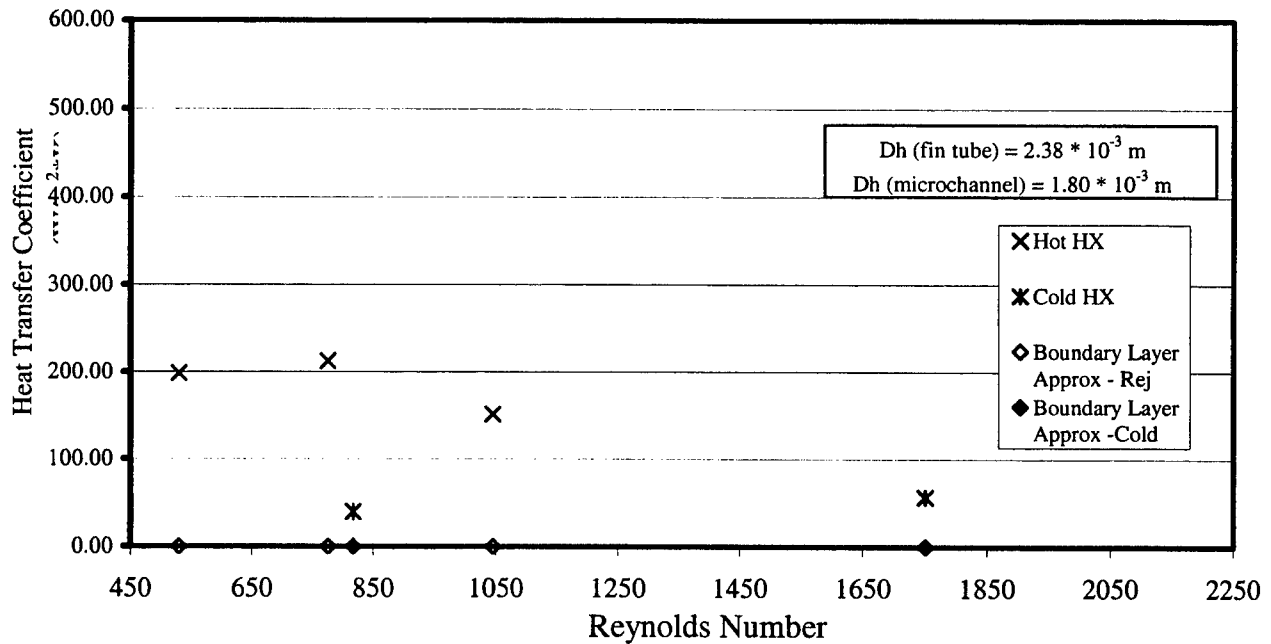
Figure 12. Heat Transfer Coefficient ( W/m^2 \cdot K ) vs. Reynolds Number for Periodic Flow; Fin-Tube Heat Exchanger
