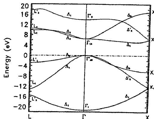
FIG. 8. The calculated electron band structure of diamond (C) along the symmetry directions \Delta and \Delta' , as obtained with the optimal basis set of the BZW procedure.
