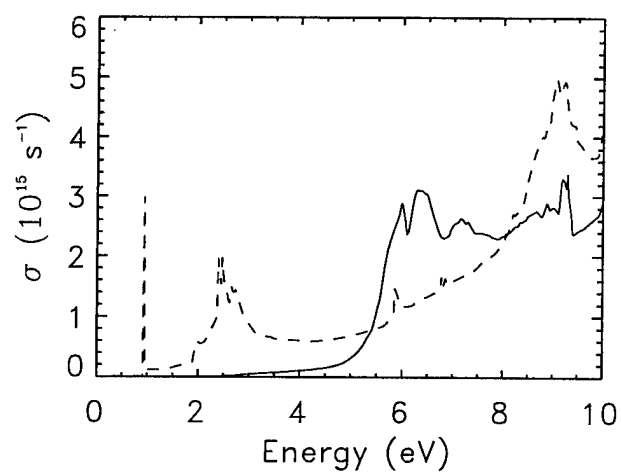
Figure 9. The calculated optical conductivity of \text{MgB}_2 . The solid line presents \sigma_{zz}(\omega) ; the dashed line presents (\sigma_{xx}(\omega) + \sigma_{yy}(\omega))/2 .
