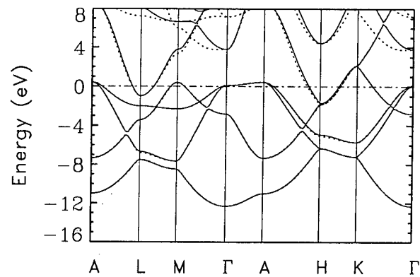
Figure 1. The comparison of the results of Calculation I and II. The solid lines represent the bands of MgB 2 from the minimum basis set calculation (Calculation I); the dashed lines show the bands from Calculation II.
