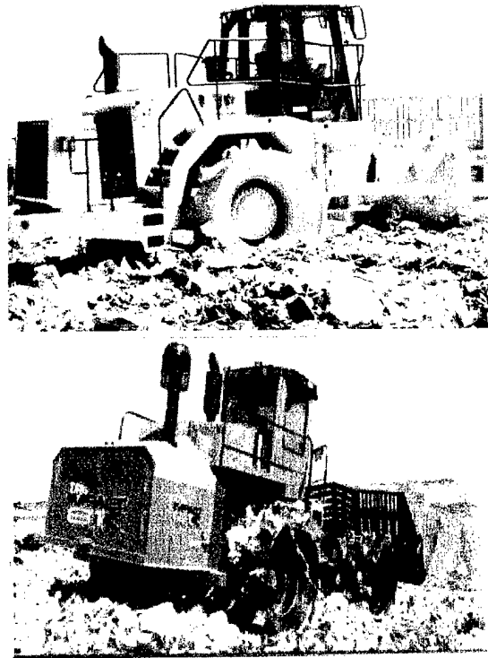
Figure 1-8: Caterpillar 826G (top) and Al-jon 81K (bottom)
