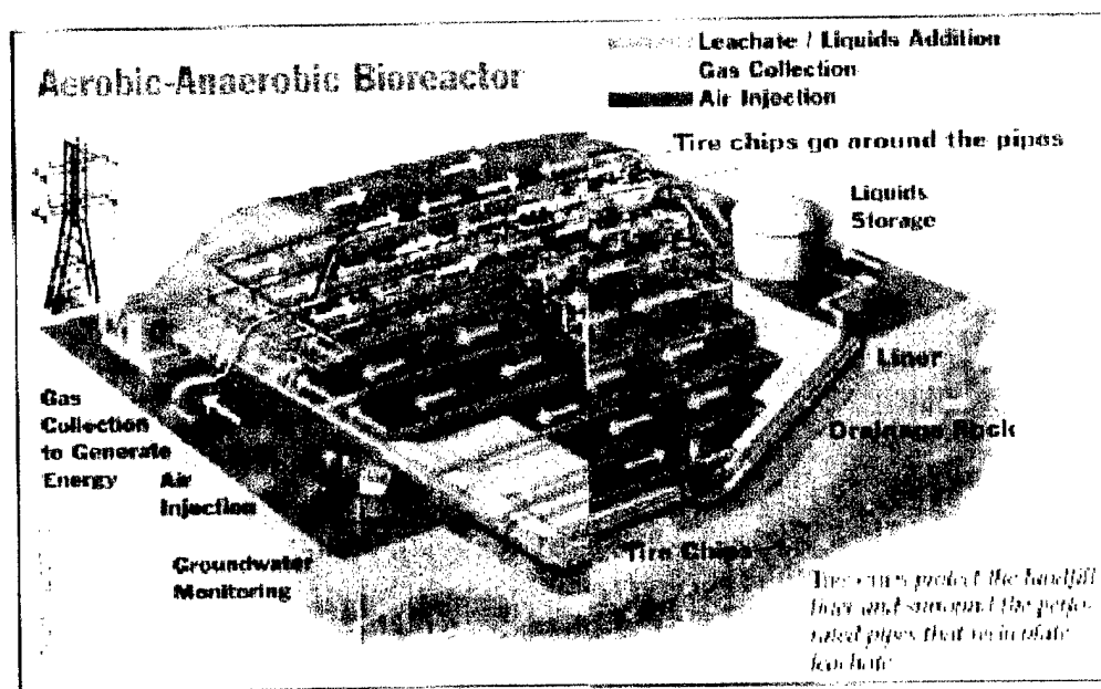
Figure 1-4: Aerobic-Anaerobic Bioreactor
