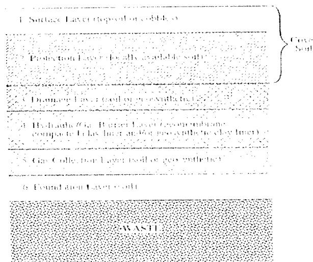
Figure 1-5: Typical Final Cover Design
