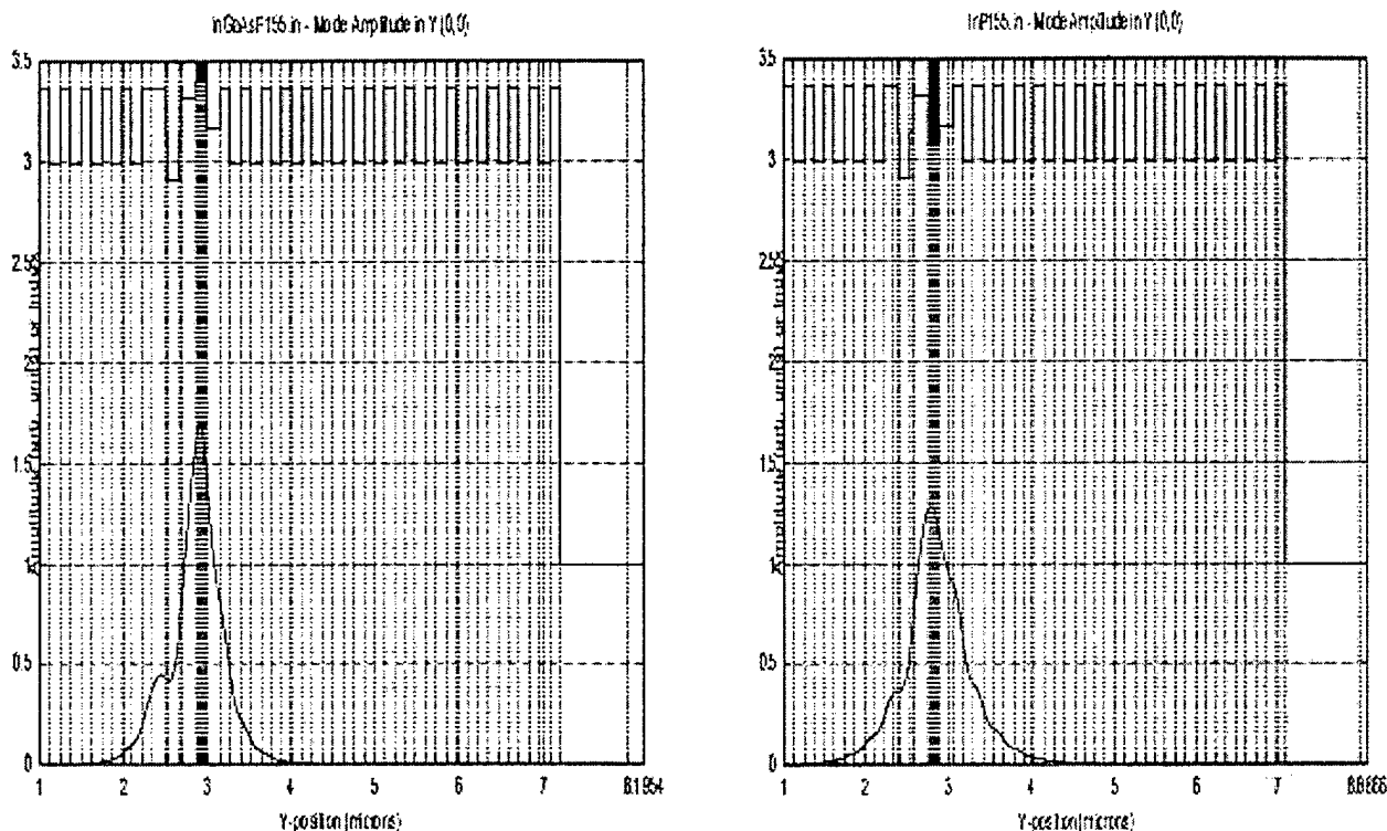
Fig. 4: The TE_{00} mode field intensity profile (a.u.) and the profile of the refractive index along the growth direction for VCSELs (a) and (b) in Fig.3.
