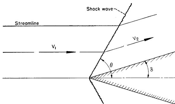
FIGURE 5.—Flow past a wedge.
