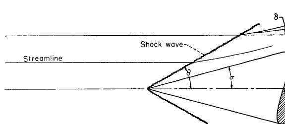
FIGURE 6.—Flow past a cone.
