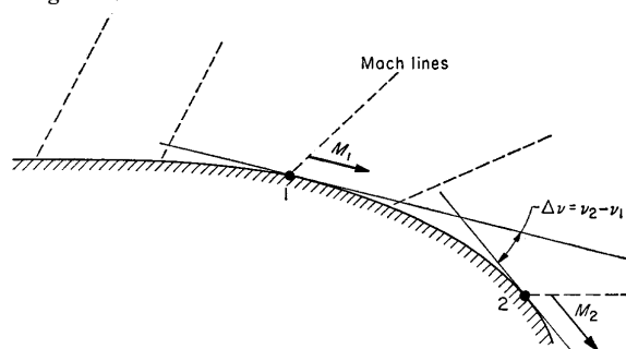
FIGURE 8.—Prandtl-Meyer expansion over a convex surface.
