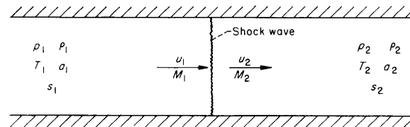
FIGURE 1.—Notation for normal shock wave.
