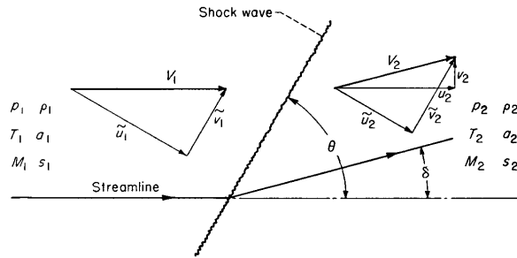
FIGURE 2.—Notation for oblique shock wave.
