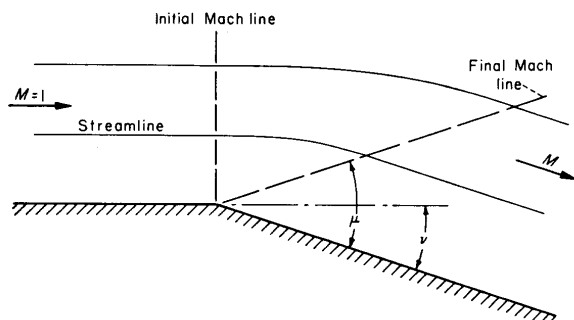
FIGURE 7.—Prandtl-Meyer expansion around a corner.
