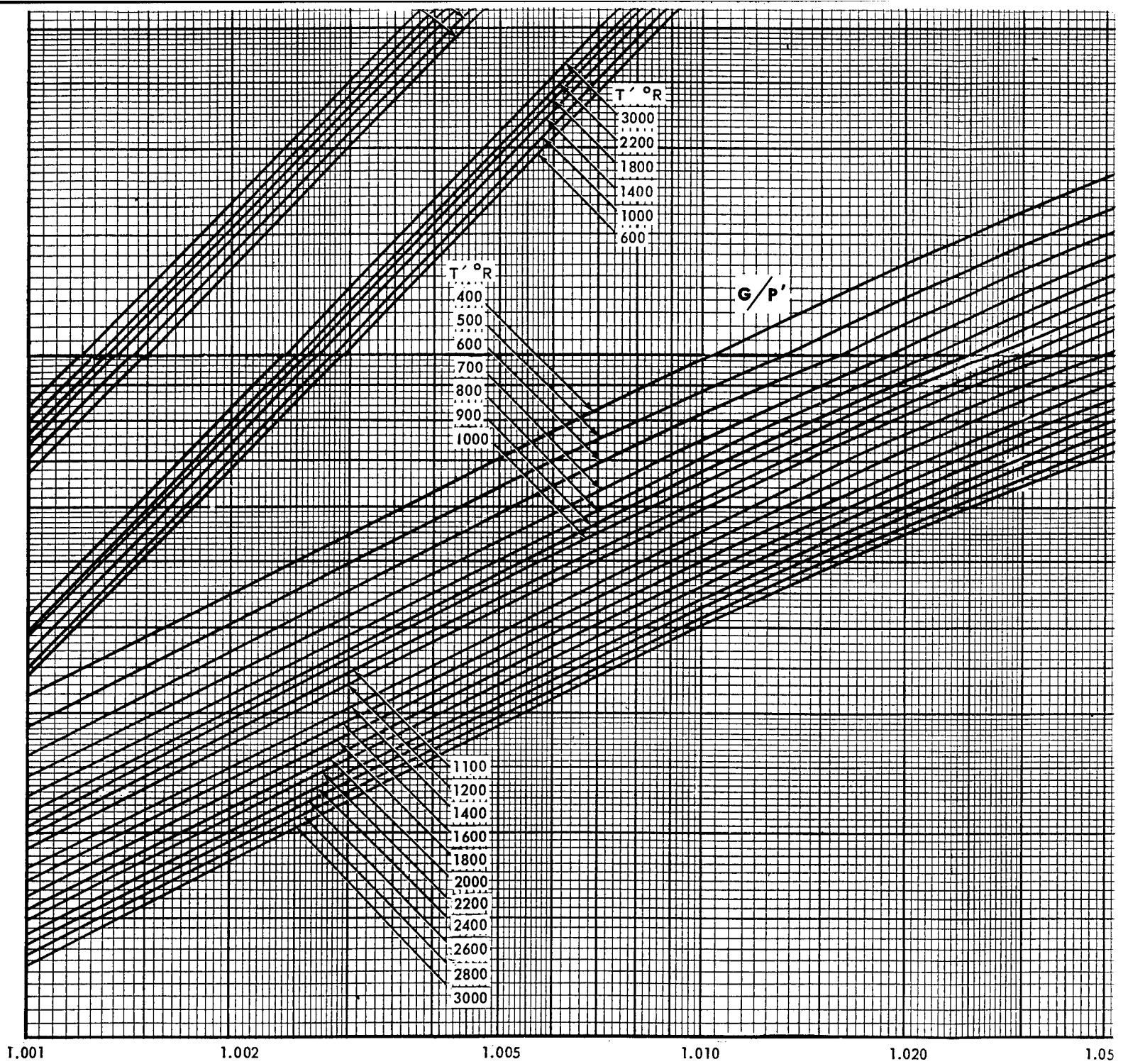
Fig. 4A - Air dynamics chart (reference data: Keenan)
