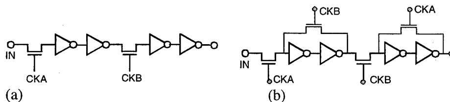
Figure 3.3 Circuit schematics of the (a) dynamic design and (b) pseudo-static design.
