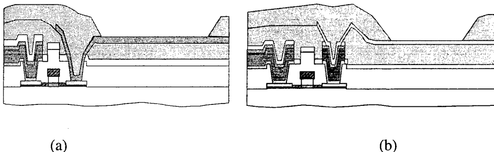
Figure 2.7 Two different processes are shown to contact the ITO to the silicided polysilicon island; (a) the ITO contacts the silicide directly, and (b) the ITO contacts a data metal plug which then contacts the silicide.
