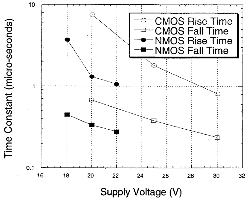
Figure 3.8 Rise and fall times of NMOS and CMOS buffers. C_{LOAD} = 30 pF
