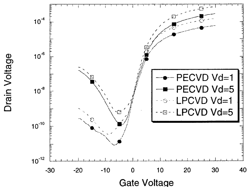
Figure 1.3 Comparison of LPCVD and PECVD deposited optimized TFTs. The LPCVD device has a mobility of 36 \text{ cm}^2/\text{V-s} and a crystallization temperature of 700^\circ \text{C} . The PECVD device has a mobility of 16 \text{ cm}^2/\text{V-s} and crystallization temperature of 605^\circ \text{C} .
