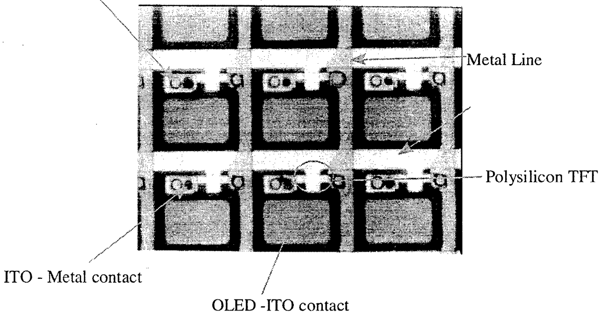
Figure 2.11 Photograph of a completed 50 μm square single TFT pixel (top view).
