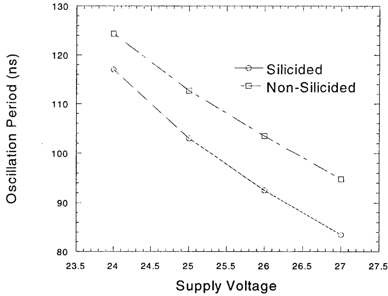
Figure 3.7 Oscillation period of a 19-stage ring oscillator as a function of the power supply voltage. The data is shown for both silicided and non-silicided ring oscillators.
