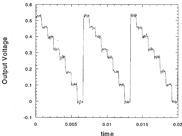
Figure 3.11 Plot of DAC output voltage as a function of time. The input bits are changed at a rate of 1.2 kHz.
