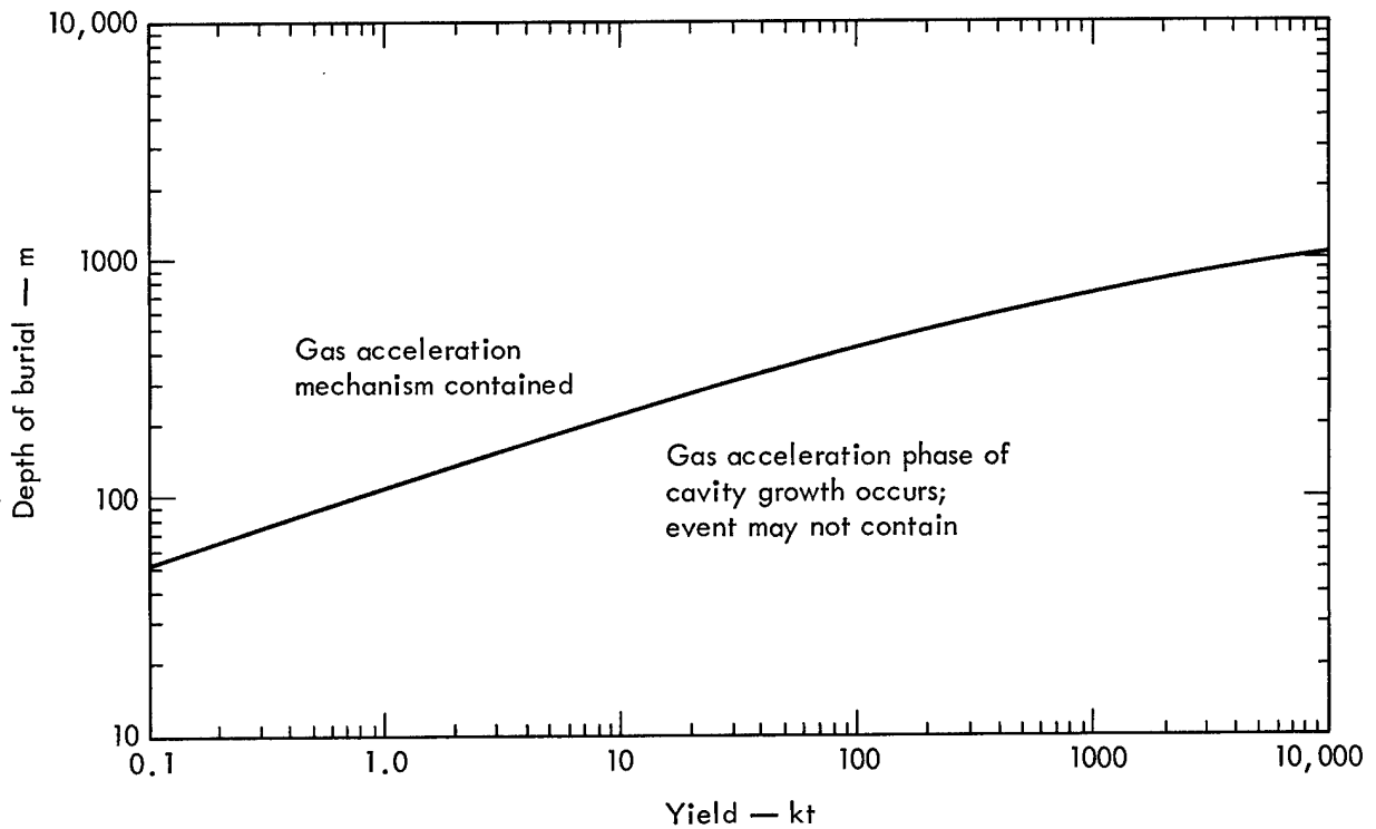
Fig. 8. Burial criterion (gas acceleration in Lewis shale).
