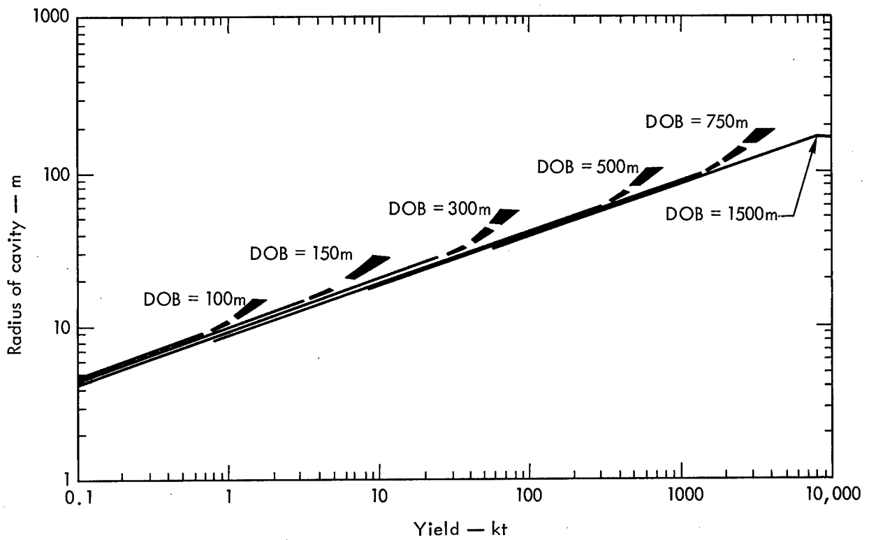
Fig. 7. Results of several series of calculations at various depths of burial (SOC parameter study in Lewis shale).
