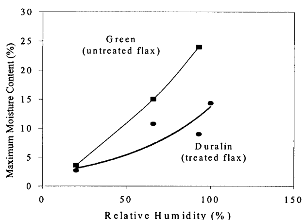
Fig. 3. The environmental relative humidity effect on the moisture absorption content of Green and Duralin flax fibers.
