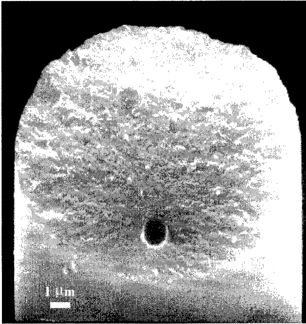
Fig. 4. SEM of fracture surface of Nextel 610 fiber from fractography testing. The fiber broke at a stress of 3.38 GPa at a 1.3 μm round, internal pore. Bar = 1 μm.
