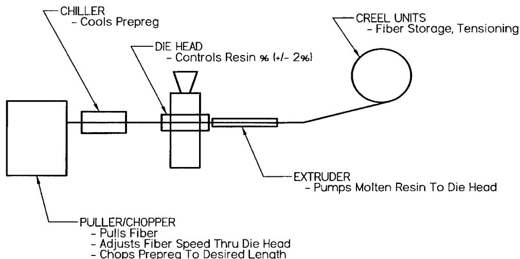
Fig. 1. DRIFT process.
