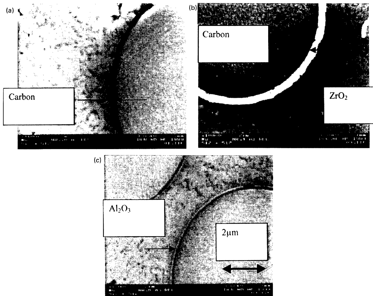
Fig. 2. Scanning electron micrographs of the interphases after hot-pressing at 1300°C for 15 min under 10 MPa pressure. (a) Reference sample; (b) carbon/ZrO 2 ; and (c) carbon/Al 2 O 3 .
