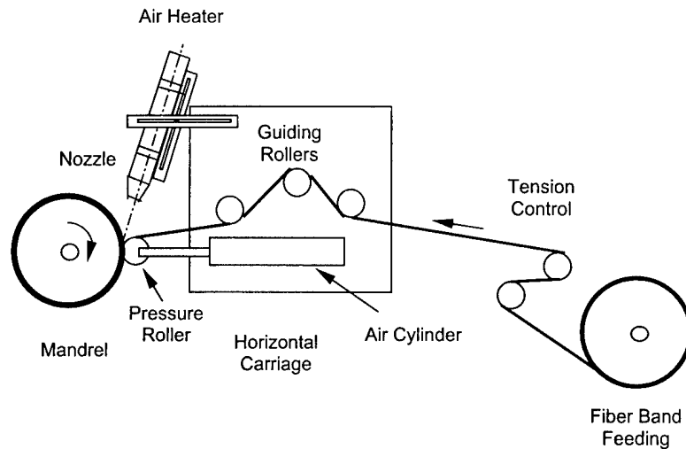
Fig. 4. Schematic diagram for on-line consolidation filament winding system.
