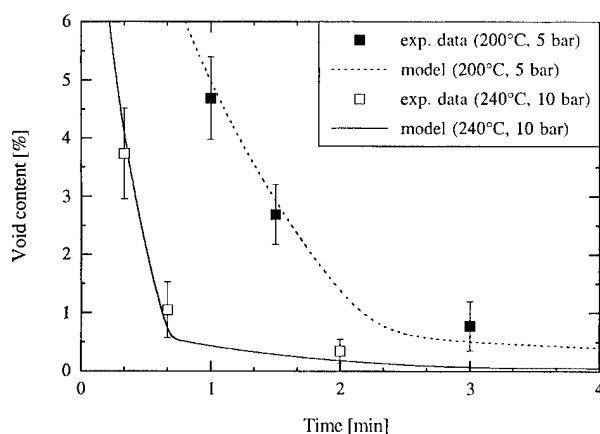
Fig. 10. Variation of void content with consolidation time for tubular braids of CF/PA12 commingled yarns processed by bladder inflation moulding.
