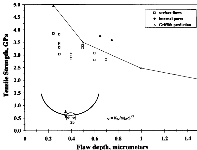
Fig. 5. Comparison of measured flaw size with the Griffith strength prediction for Al 2 O 3 fibers ( K_{Ic} = 2.8 ) with semicircular surface flaws. Flaw size must be well below 1 μm to achieve 3 GPa strength. Measured flaw size, a , was slightly less than the predicted strength for surface flaws, but above the prediction for round, internal pores.
