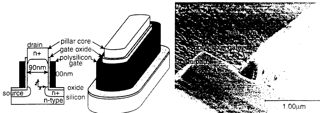
Figure 3: a) Diagram of depletion-mode fin surrounding-gate transistor. b) SEM image in oblique view of gated depletion-mode fin surrounding-gate transistor before passivation.
