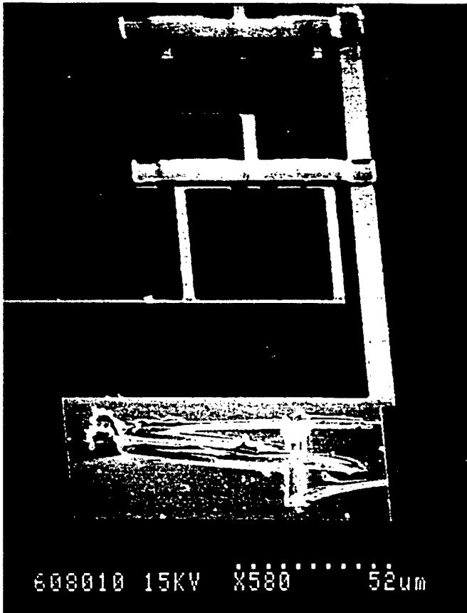
Fig 3: Dual anchor
