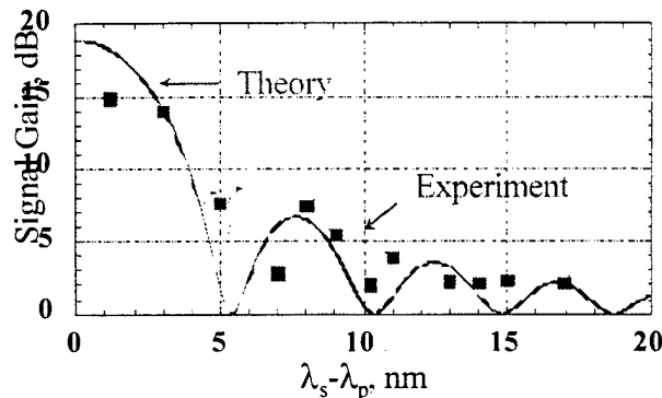
Figure 1: Experimental results for an FWC using HNLF.
