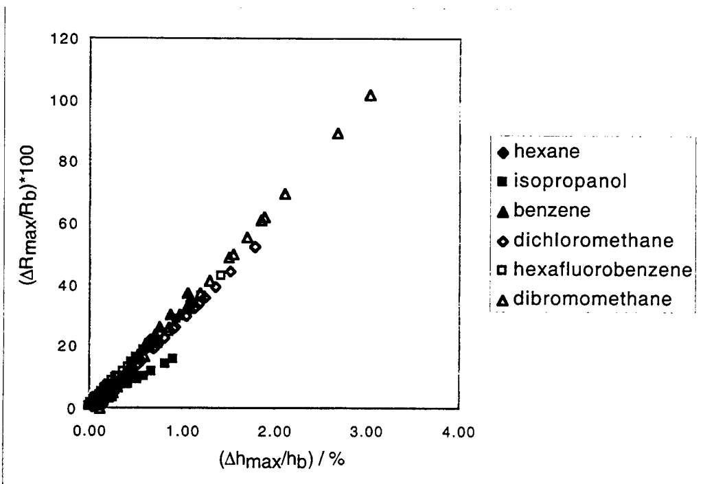
Figure 23. Relative resistance increase for a PCL-carbon black composite film verses relative thickness increase for a PCL clear film when both films were exposed to various analytes at various fractional vapor pressures, correlated by the analyte fractional vapor pressure for two separate (a & b) PCL films.
