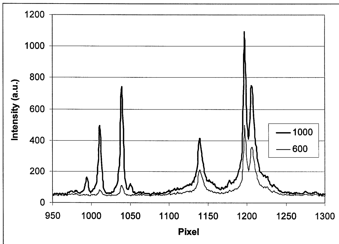
Figure 2.9: Spectral Comparison of 600 \mu\text{m} and 1000 \mu\text{m} Fiber Optics
