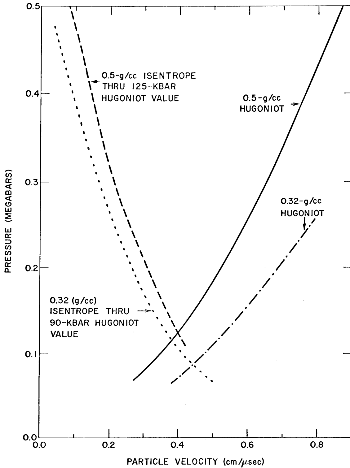
Fig. 3. The calculated BKW Hugoniots and isentropes for 0.5- and 0.32-g/cc polyurethane.
