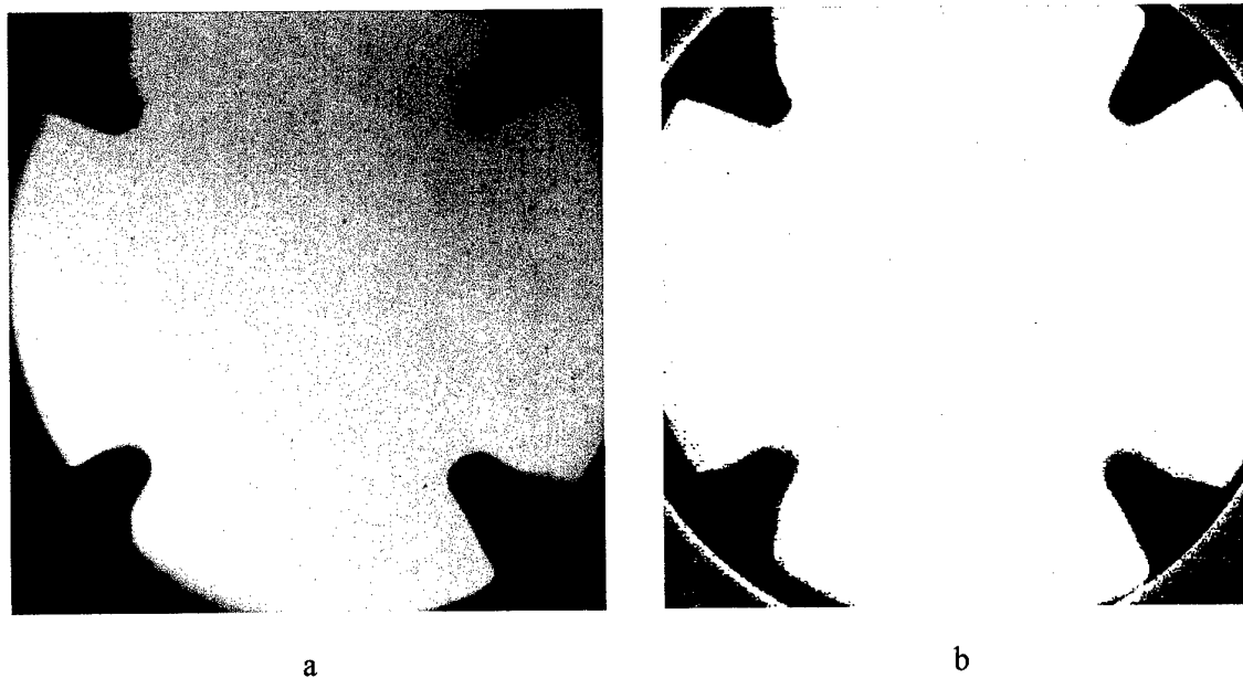
Fig.2. Image of LPS sample luminescence at the pressure p=0.1\text{bar} (a) and its ratio to the image at the pressure p=1\text{bar} (b).
