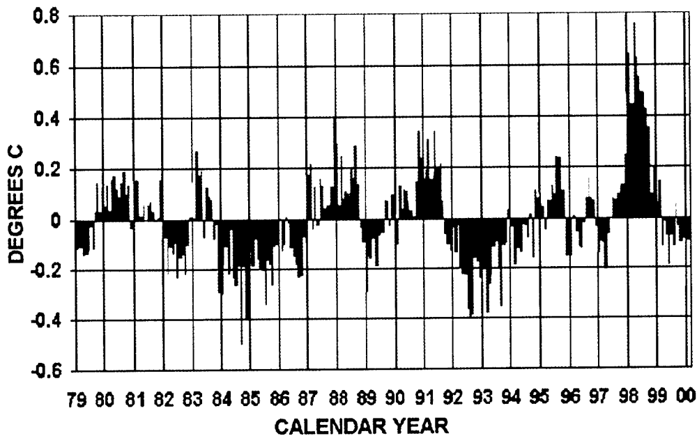
Global Tropospheric Temperature Anomalies, January 1979 - February 2000 (Christy et al., 2000)
