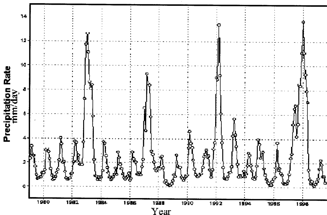
Precipitation (5N-5S, 170W-120W), 1979-1998 (Gruber, 2000)
