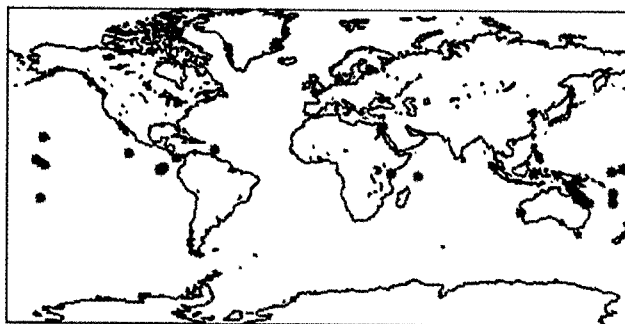
Coral Data at 1 U.S. Site and 61 Global Sites
