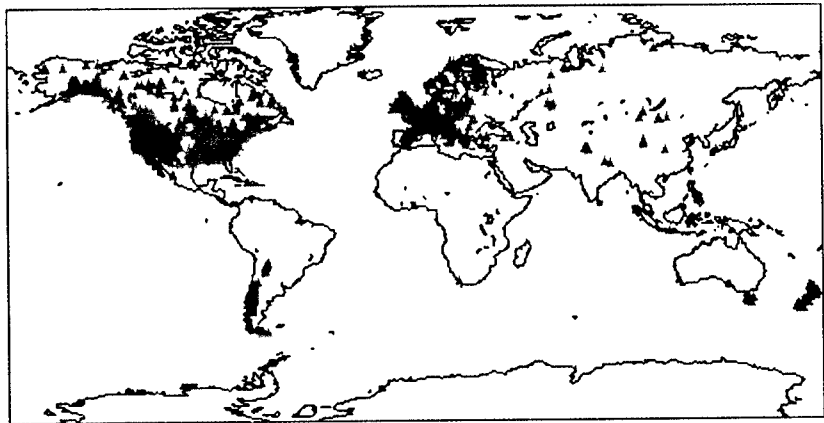
Tree Ring Data at 1029 U.S. Sites and 1854 Global Sites
