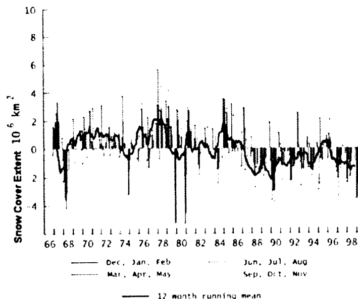
Northern Hemisphere Snow Cover Anomaly (Robinson, 2000)
