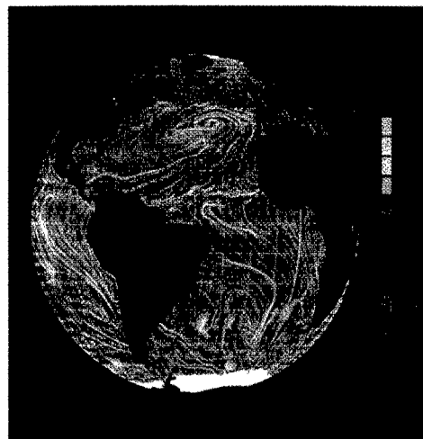
Ocean Surface Winds by QuikSCAT, August 1, 1999
