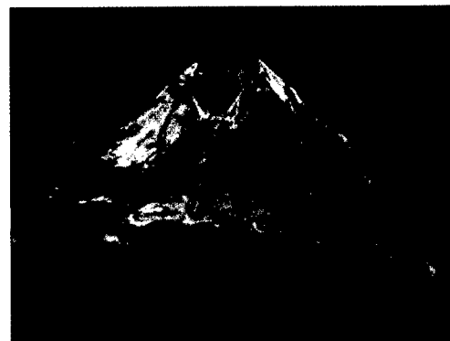
Terra/ASTER Image of Mount St. Helens Volcano, Washington State, August 2000
