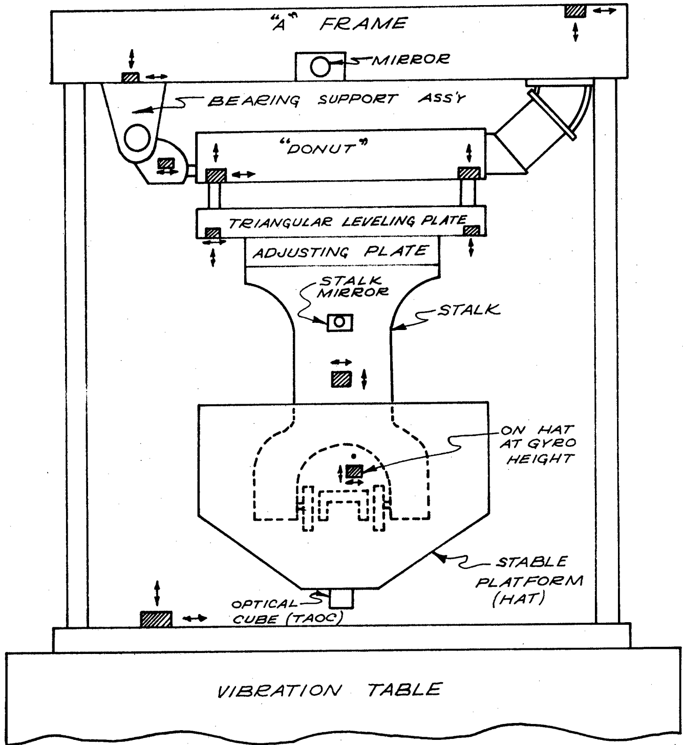
LOCATION OF VIBRATION PICKUPS ON N7F STABLE PLATFORM ASSEMBLY, SHOCKMOUNT STRUCTURE, & TEST FIXTURE
