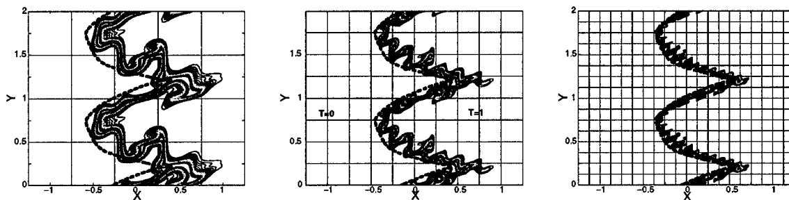
Figure 3: Direct numerical simulations to verify asymptotic convergence to the predicted front (see [6])
