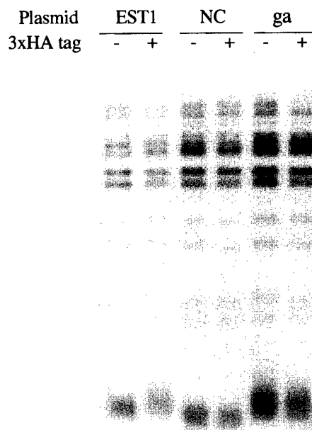
FIG. 7. The est1 mp1 nc mutant has a dominant short-telomere phenotype. Genomic DNA from an EST1 W303 \alpha strain also expressing plasmid-borne EST1 or est1-mp1-nc or est1-mp2-ga from the ADH1 promoter (pJZ-3HA- EST1 and derivatives) was digested with Xho I and analyzed by Southern blotting with ^{32} P-labeled TELPG as a probe.
