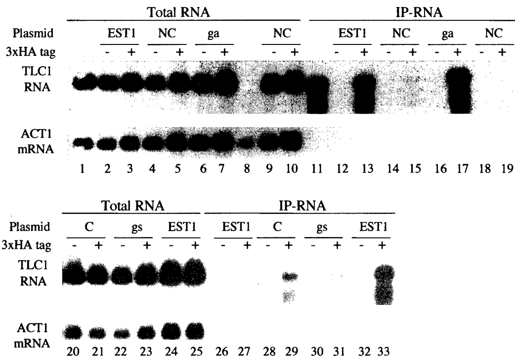
FIG. 6. Association of Tlc1 RNA with Est1 RRM mutant proteins in vivo. Total RNA and immunoprecipitated RNA (IP-RNA) were made from est1 cells expressing wild-type or mutant forms of either untagged (–) or 3HA-tagged (+) Est1 from the ADH1 promoter (plasmid pJZ-3HA-EST1 and derivatives). The amounts of Tlc1 RNA and ACT1 mRNA in total RNA or coimmunoprecipitated with Est1 were assayed by Northern blotting. Two independent transformants of Est1-RNP1-NC were assayed. Controls included RNA from a tlc1 deletion mutant (lane 8), RNA from a strain carrying 3HA-tagged Est1 expressed from the genomic EST1 locus (lanes 1 and 11), and IP-RNA treated with RNase A before loading (lanes 26 and 27).
