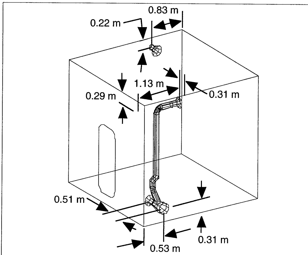
Figure 8. Ventilation System Schematic
