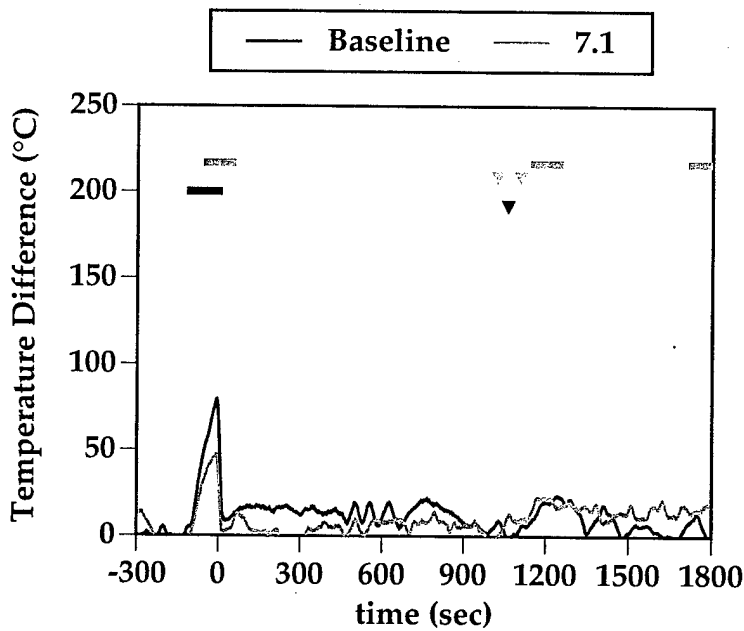
Figure C-1. Fire Plume and Compartment Temperatures for Test 7.1 vs. Baseline
