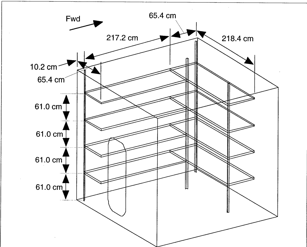
Figure 6. FLSR 1 Storage Shelves
