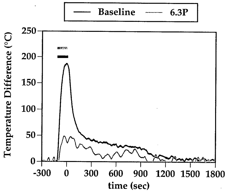
Figure A-3. Fire Plume and Compartment Temperatures for Test 6.3P vs. Baseline (Subgroup A)
