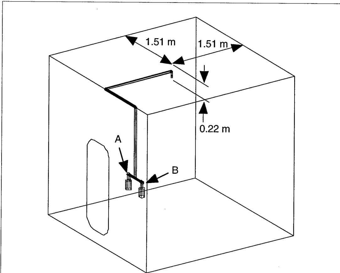
Figure 11. FLSR 1 Gaseous Suppression Agent Distribution System Schematic
