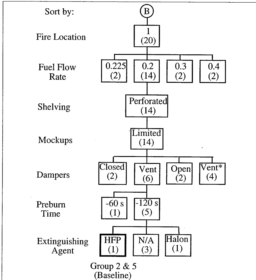
Figure 21C. FLSR 1 Tests
