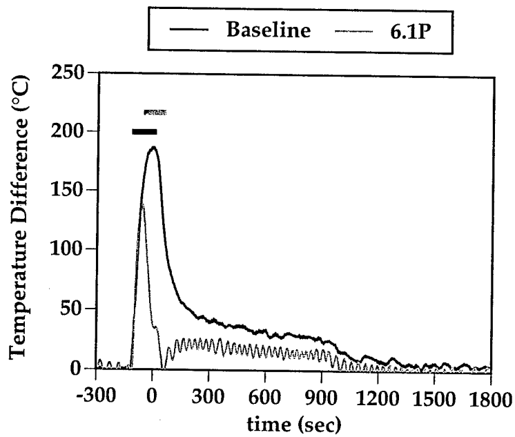
Figure A-1. Fire Plume and Compartment Temperatures vs. Baseline for Test 6.1P (Subgroup A)
