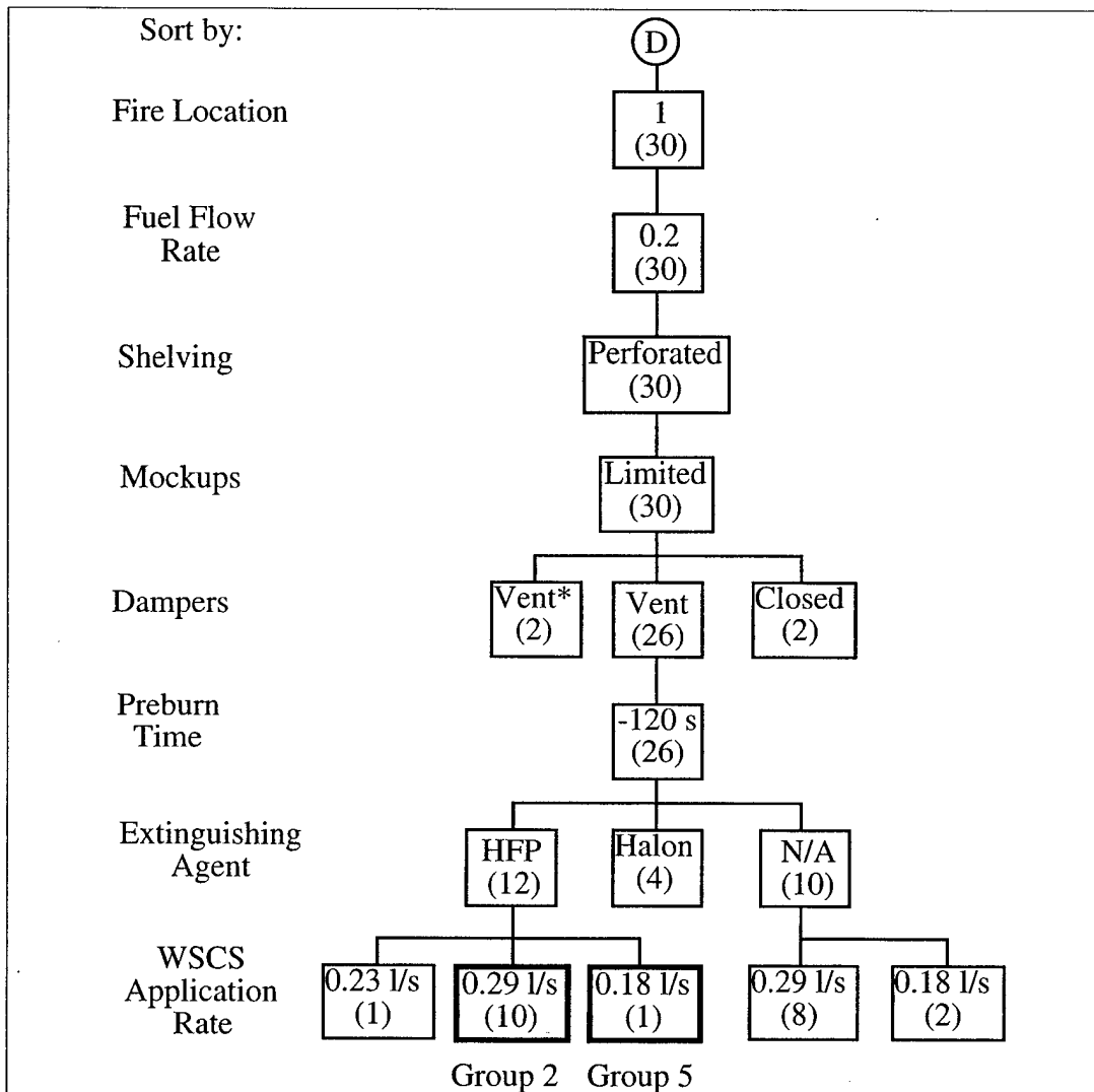
Figure 21E. FLSR 1 Tests
