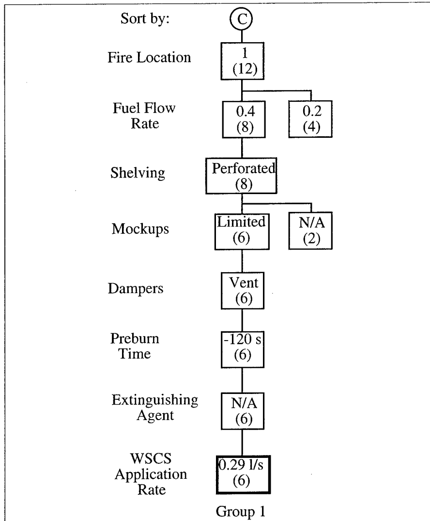
Figure 21D. FLSR 1 Tests
