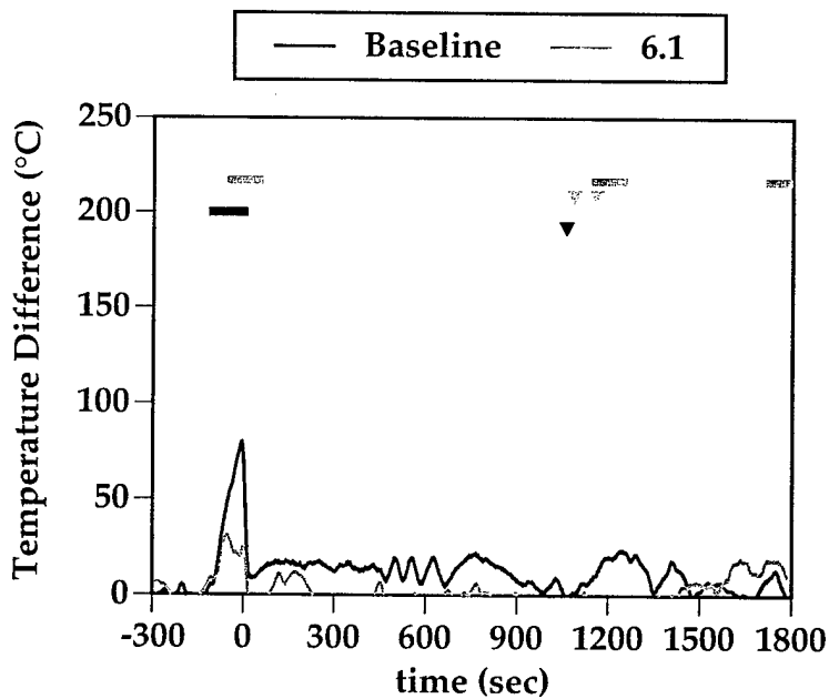
Figure B-1. Fire Plume and Compartment Temperatures vs. Baseline for Test 6.1
