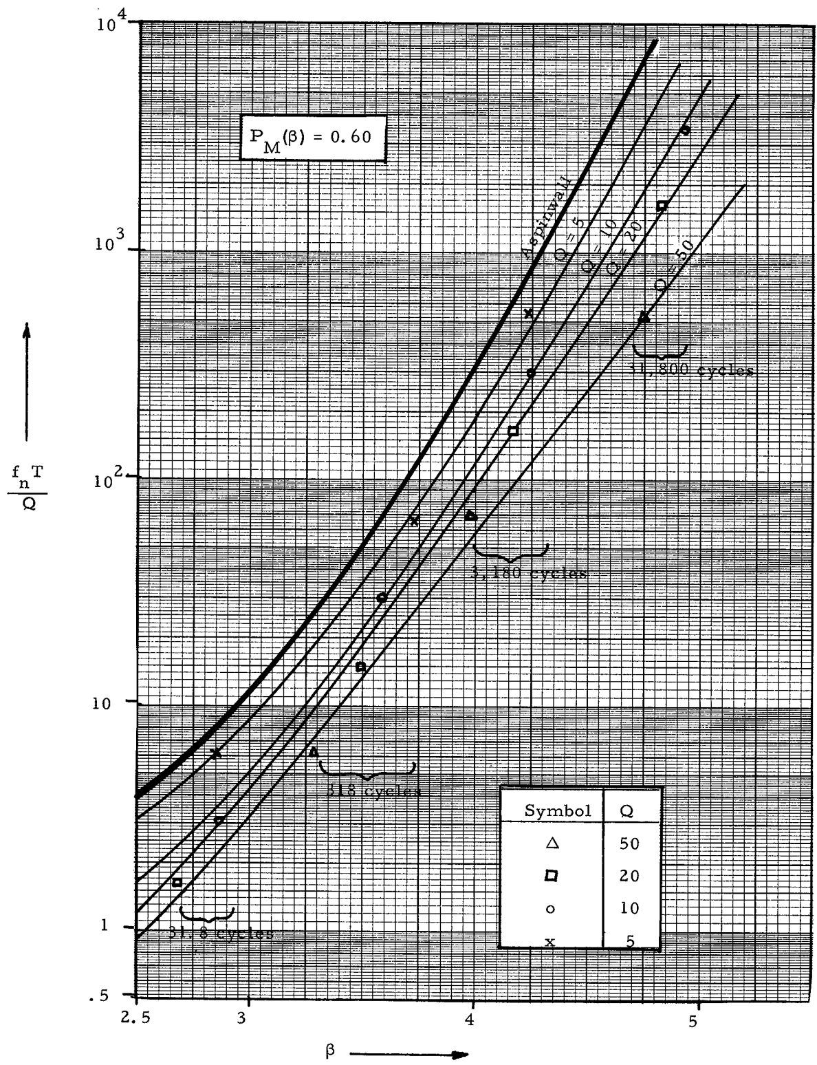
Figure 7. Dimensionless Time Parameter Versus the Ratio of Peak to RMS Response for the Output of a Mechanical Oscillator Excited by Stationary White Noise: P_M(\beta) = 0.60
