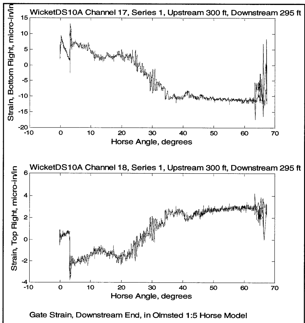
Figure 68. Gate strain, downstream end – bottom-lifted, 2-gate gap
