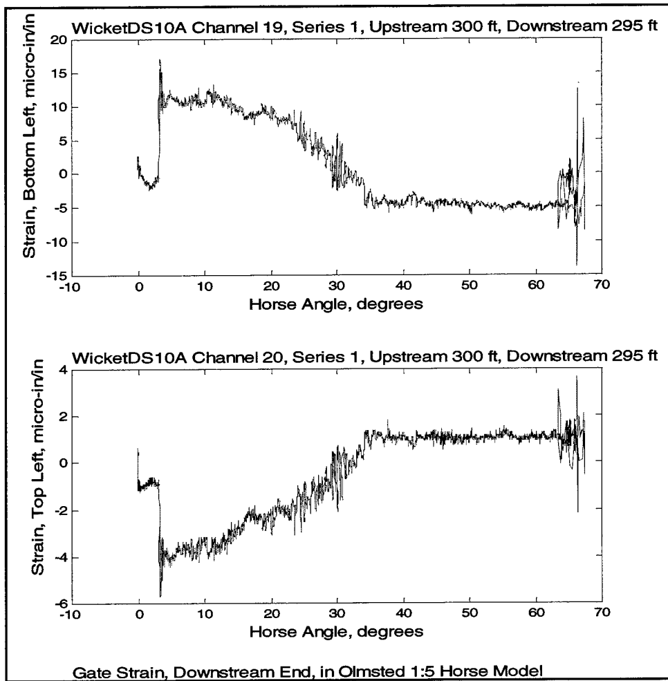
Figure 69. Gate strain, downstream end – bottom-lifted, 2-gate gap
