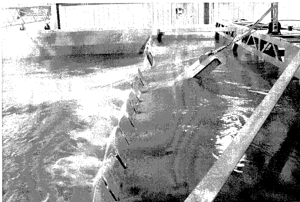
Figure 24. Pool el 300, tailwater el 295. View looking from left side. Cable attached to bottom of gate. Gate raising, gate position just prior to prop-rod setting in hurter
