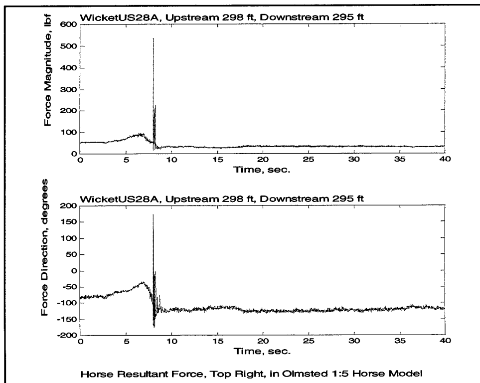
Figure C38. Horse resultant force, top right-Bottom-lift drop test-no gap (WicketUS28A)
