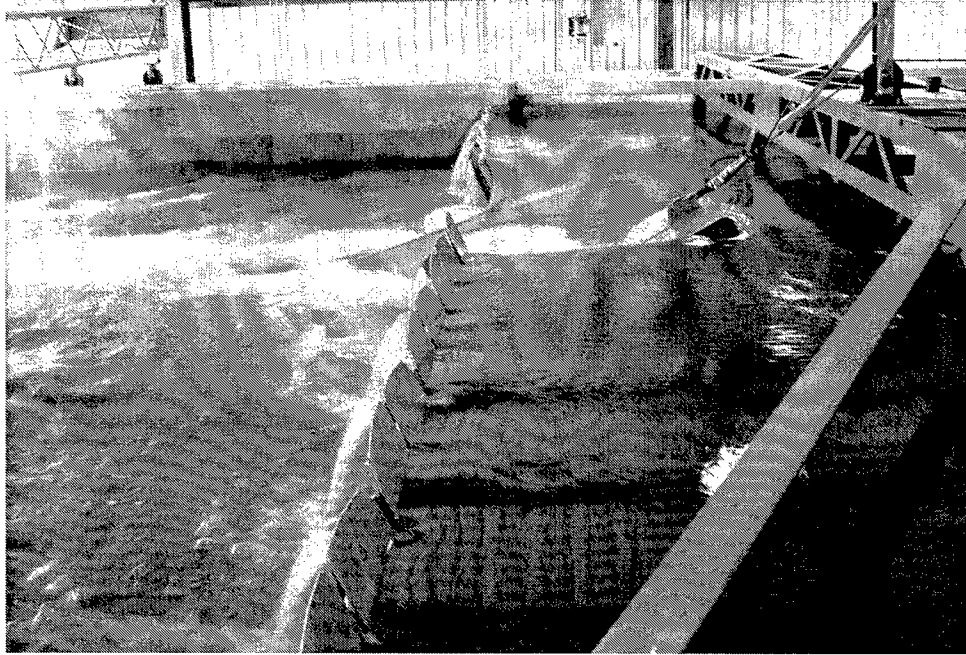
Figure 25. Pool el 300, tailwater el 295. View looking from left side. Cable attached to bottom of gate. Gate raising, gate position with prop-rod set in hurter
