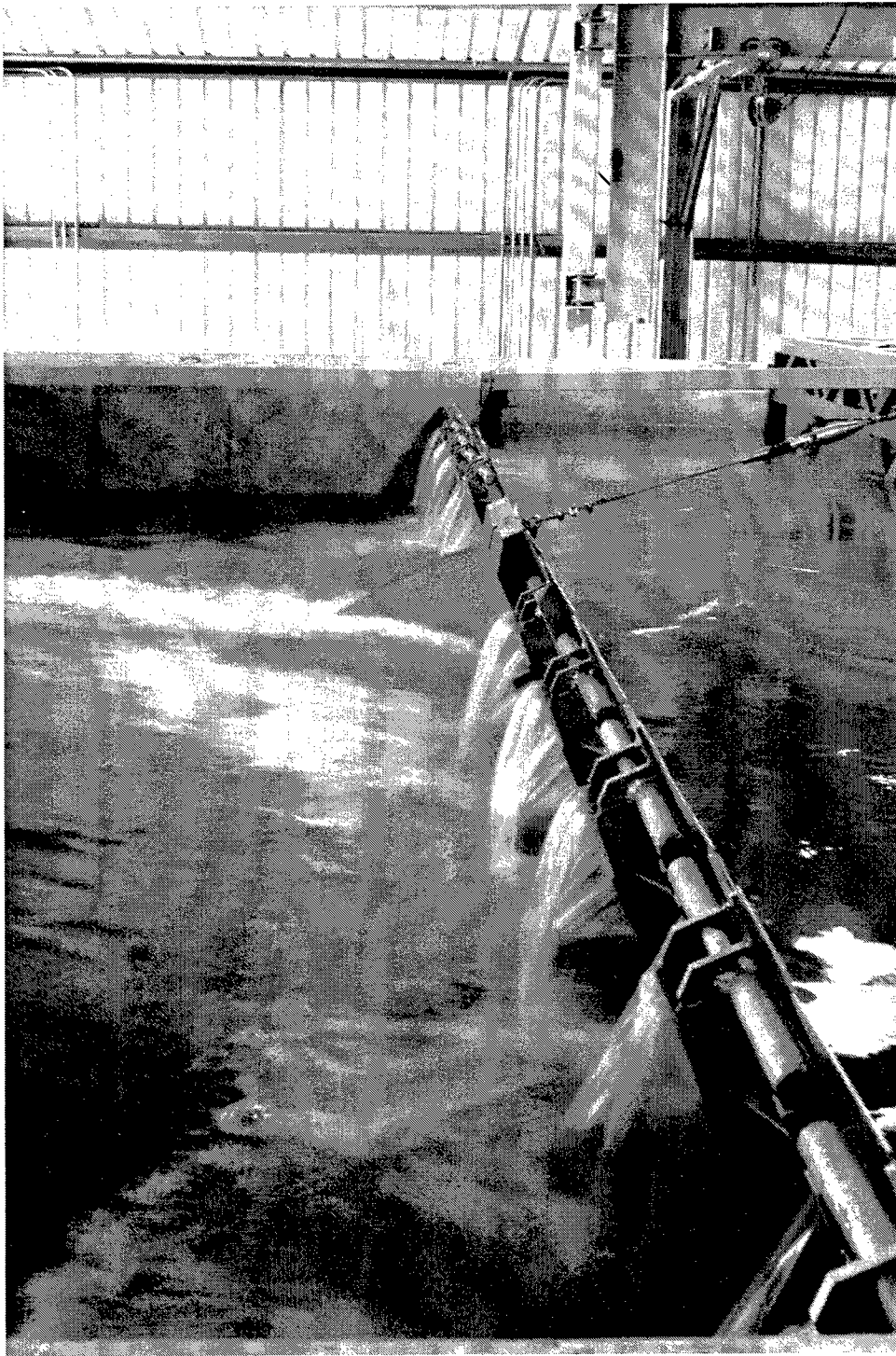
Figure 20. Pool el 300, tailwater el 295. View looking from left side. Cable attached to top of gate. Gate in operating position at 65 deg
