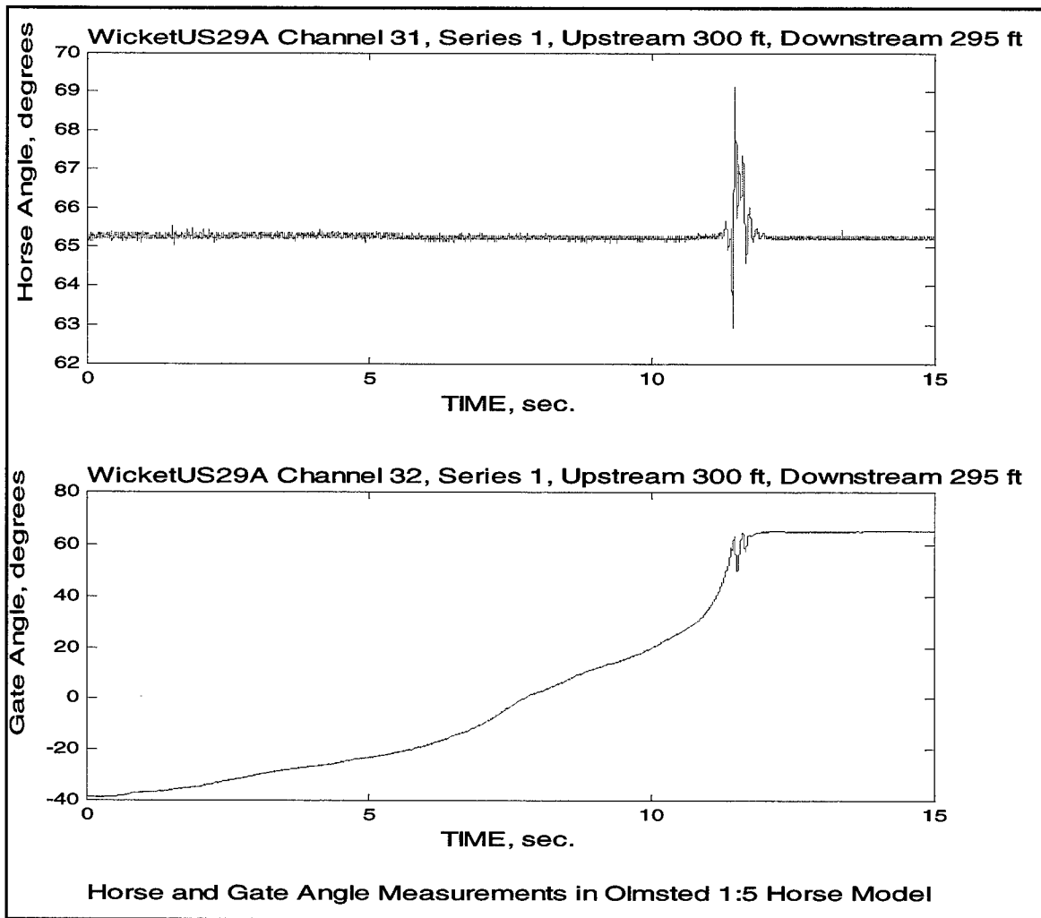
Figure 119. Gate and horse angle during the flipping operation— bottom-lift drop test, no gap
