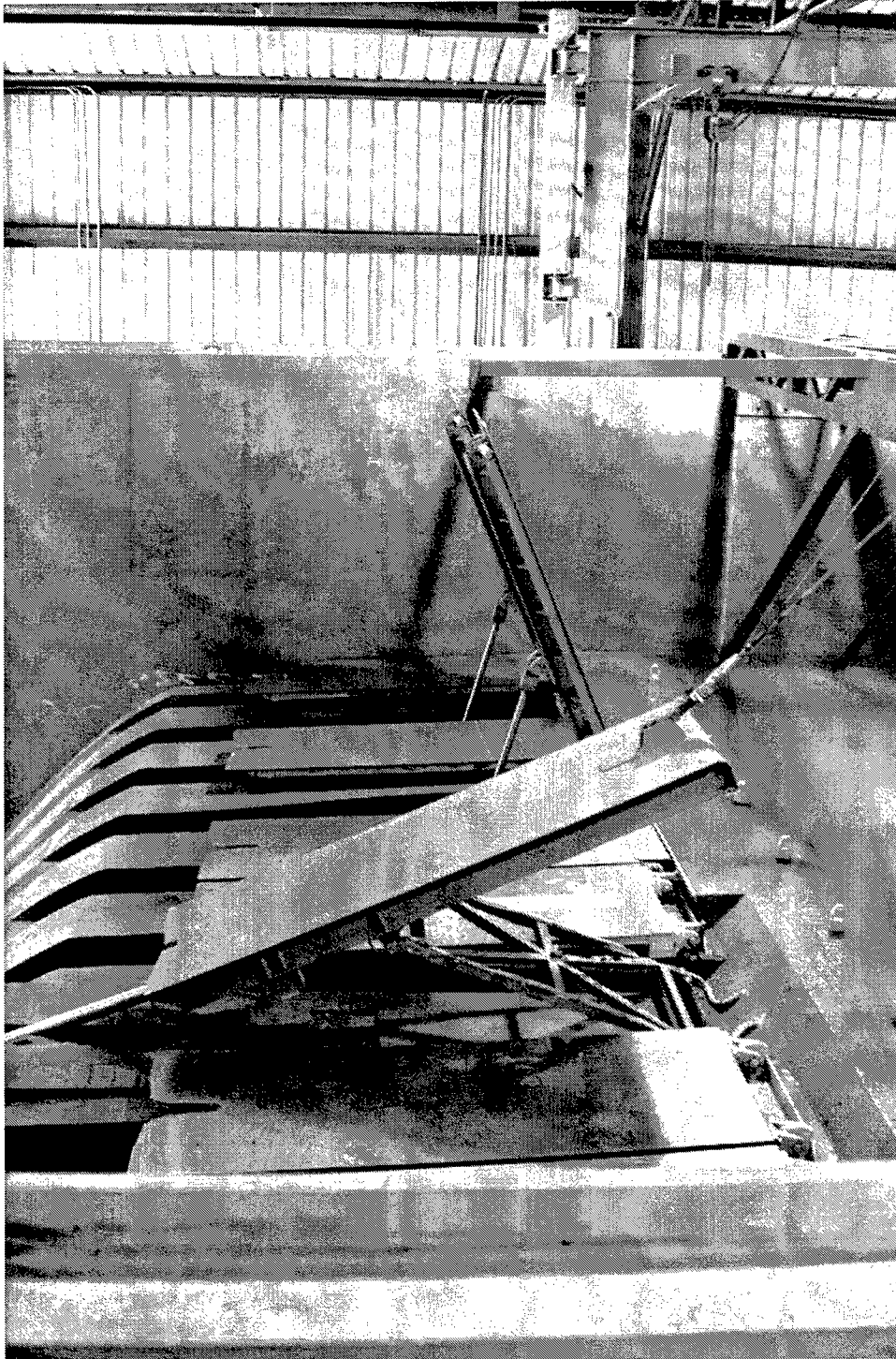
Figure 8. Dry bed view looking from left side. Cable attached to bottom of gate. Gate near lowered position
