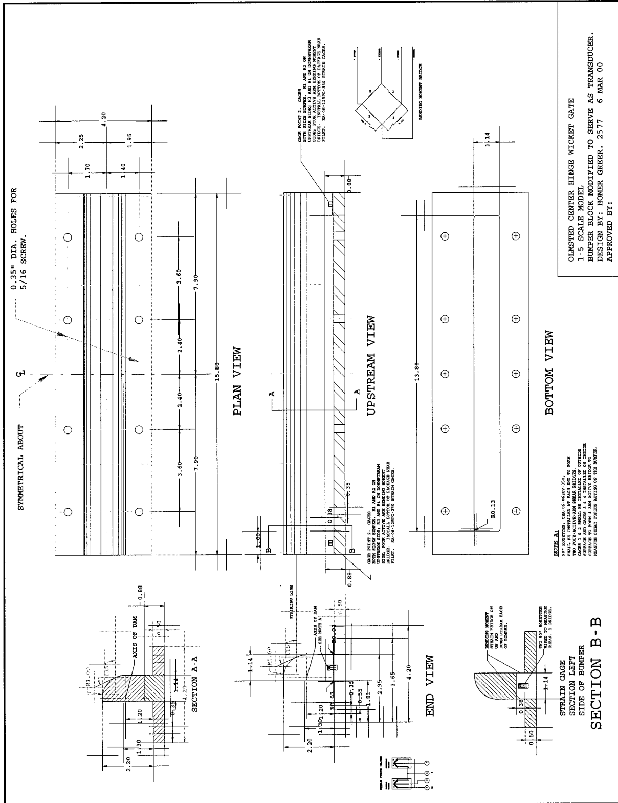
Figure 32. Strain gage locations on the modified bumper block for measuring the impact stresses resulting from drop test
