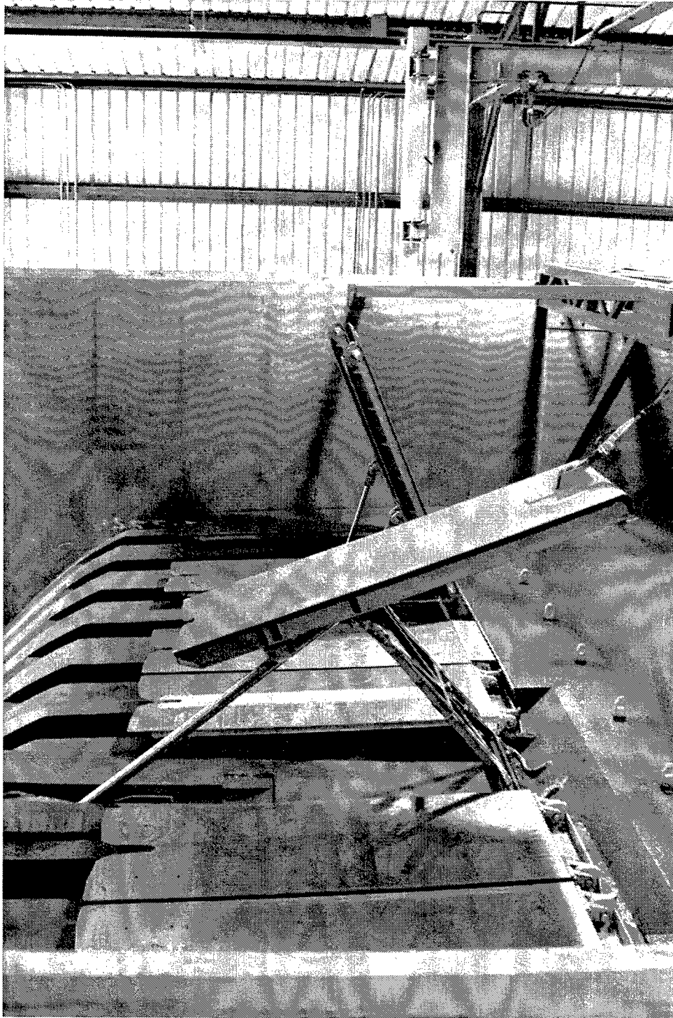
Figure 7. Dry bed view looking from left side. Cable attached to bottom of gate. Gate position near start of lowering operation
