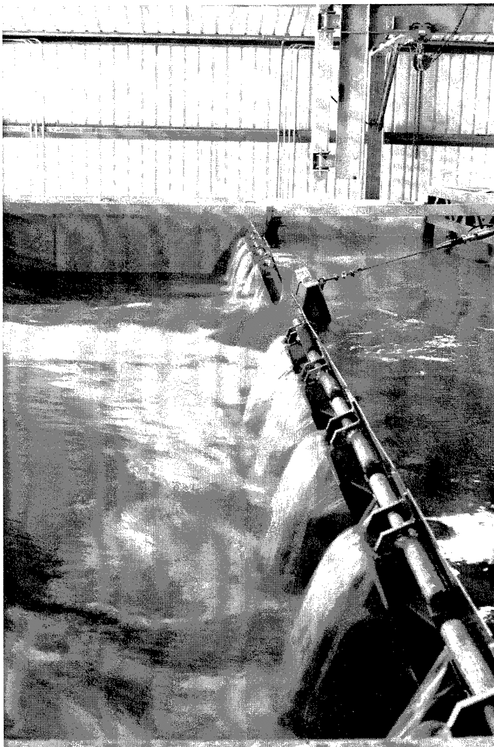
Figure 18. Pool el 300, tailwater el 295. View looking from left side. Cable attached to top of gate. Gate position near 70 deg
