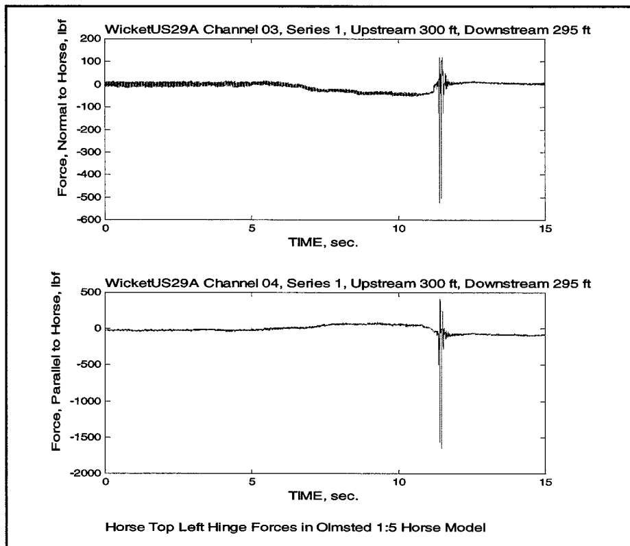
Figure C2. Bottom-lift drop test-no gap (WicketUS29A)
