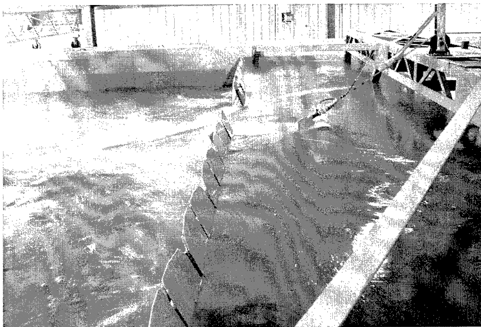
Figure 23. Pool el 300, tailwater el 295. View looking from left side. Cable attached to bottom of gate. Bottom of gate near water surface
