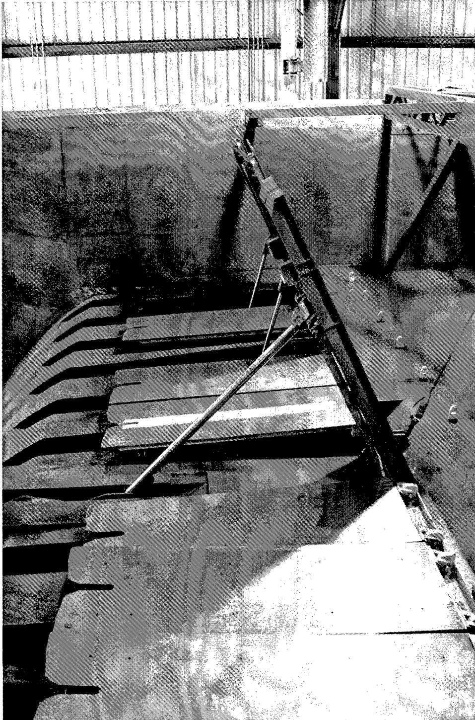
Figure 4. Dry bed view looking from left side. Cable attached to bottom of gate. Gate raised to 65 deg
