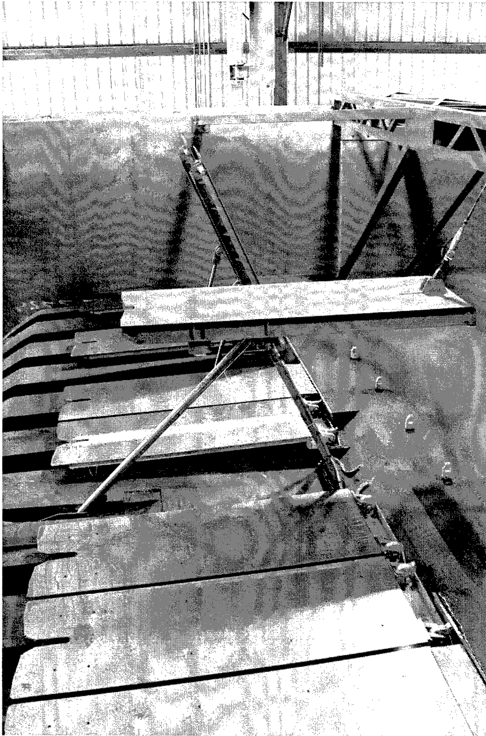
Figure 5. Dry bed view looking from left side. Cable attached to bottom of gate. Prop-rod set in hurrer. Gate pivoted in horizontal position to 0 deg
