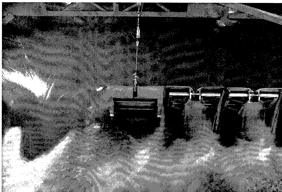
Figure 21. Pool el 300, tailwater el 295. View looking upstream. Cable attached to top of gate. Gate in operation position at 65 deg
