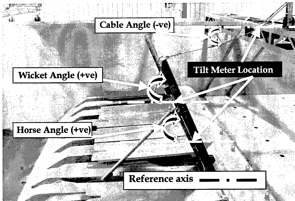
Figure 36. Angular orientation of tilt meter measurements
