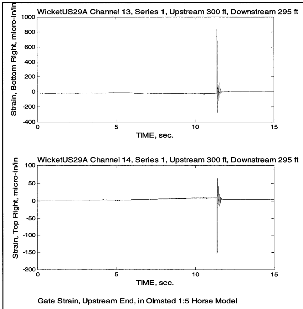
Figure C9. Gate strain-upstream end-Bottom-lift drop test-no gap (WicketUS29A)
