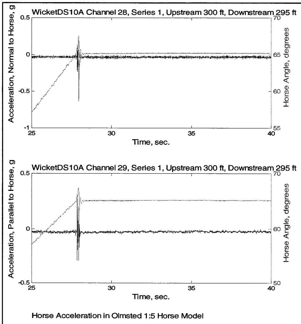
Figure 76. Horse acceleration when the prop rod was positioned on the hurter – bottom-lifted, 2-gate gap
