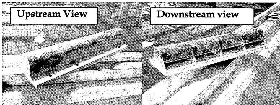
Figure 13. Rear and front view of the bumper block
