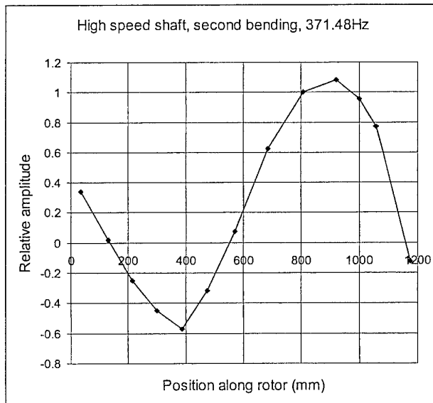
Figure 14. Second bending mode of the N2 shaft, at 371.48 Hz
