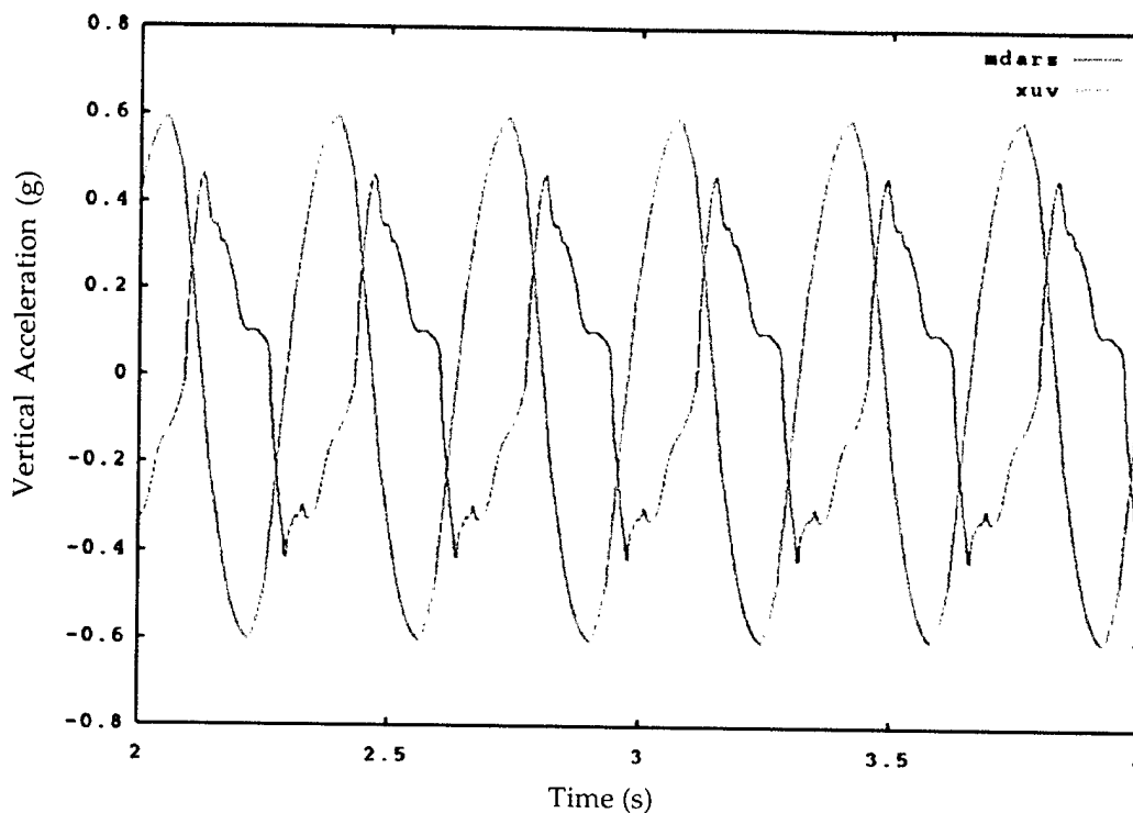
Figure 25. Chassis Vertical Acceleration, 2-Inch Washboard, 4 mph.
