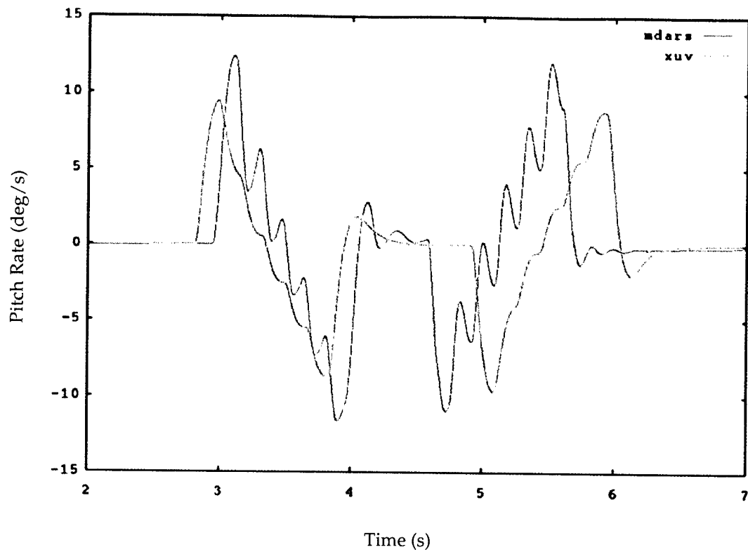
Figure 9. Chassis Pitch Rate, 3-Inch Bump, 2 mph.
