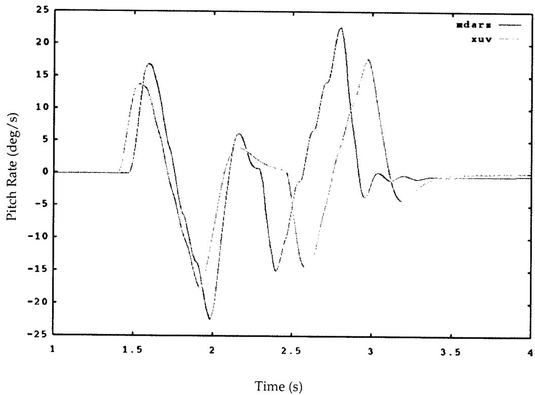
Figure 10. Chassis Pitch Rate, 3-Inch Bump, 4 mph.
