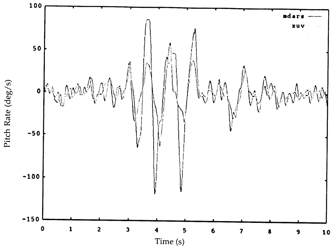
Figure 31. Chassis Pitch Rate, T101, 8 mph.
