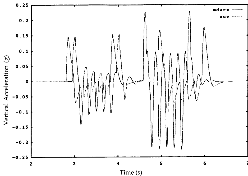
Figure 14. Chassis Vertical Acceleration, 3-Inch Bump, 2 mph.
