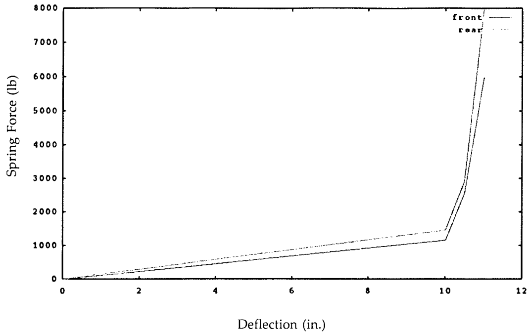
Figure 6. XUV Spring Curves.
