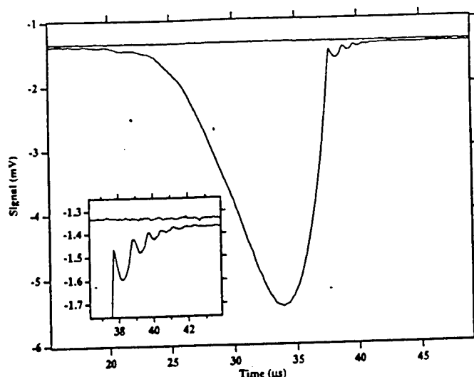
Fig. 8. Signal V(t) and noise level \bar{V}(t) for light scattered by a sonoluminescing bubble during one cycle of the driving sound field. The inset blows up the difference between signal and noise. These data show more detail than Fig. 1 because it is the average of 512 as compared to 32 sweeps.
