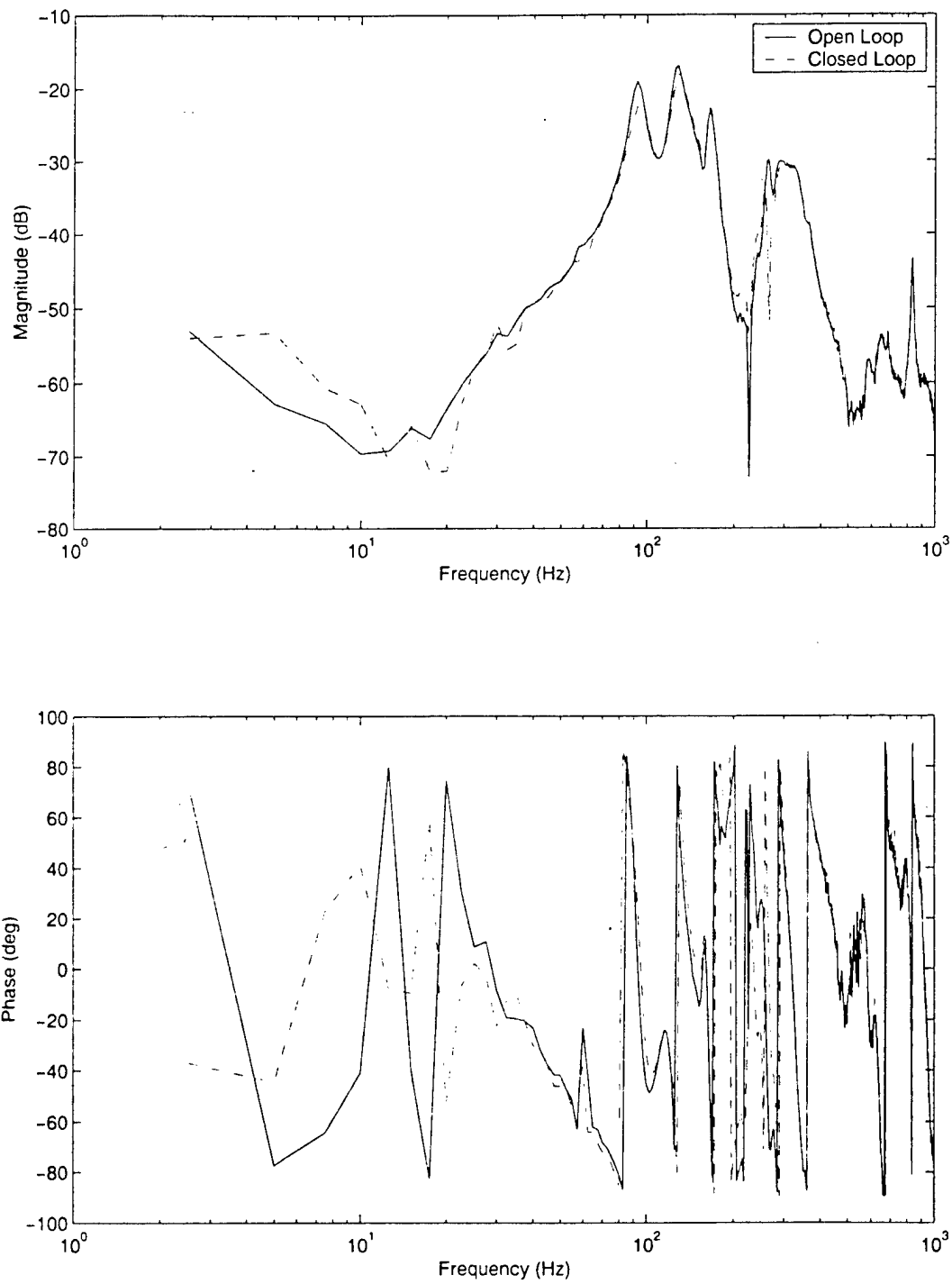
Figure 5-32: Power Diode Controller Performance (Bottom Plate System On Only)
