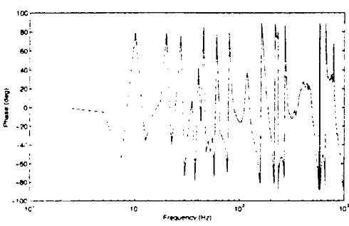
G_{y1u1} : PZT1-to-Mic1
