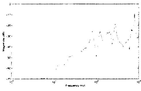
G_{y1u1} : PZT1-to-Mic1
