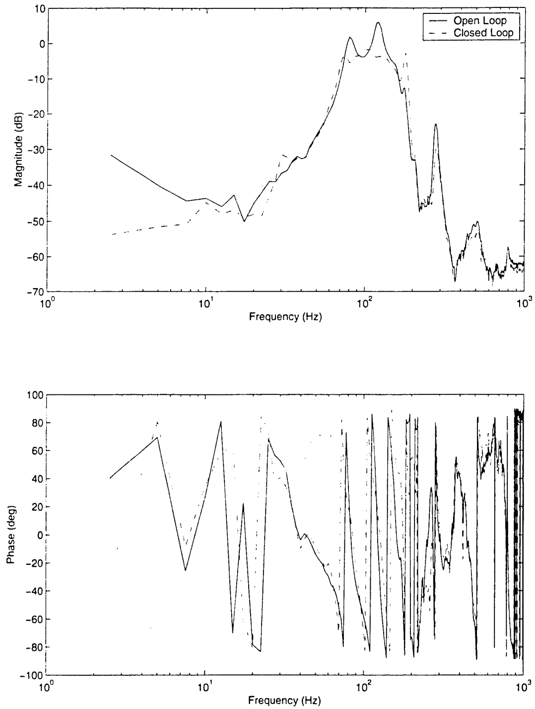
Figure 5-16: Successive Loop Closure Controller Performance (Both On)
