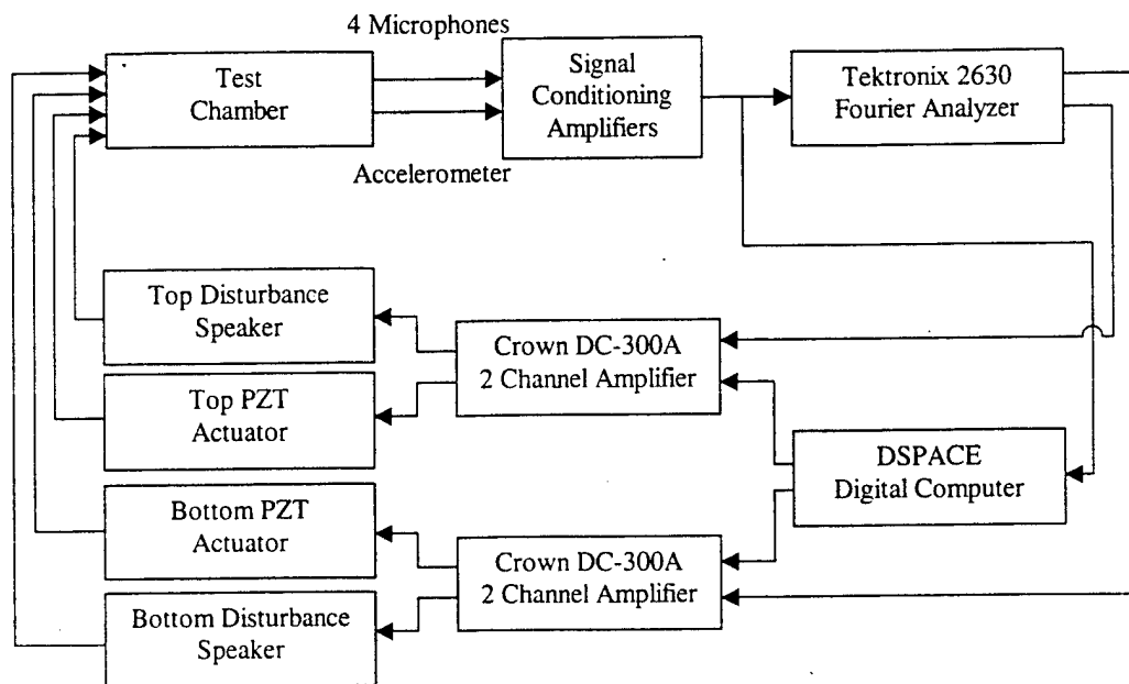
Figure 2-6: Block Diagram of the Experimental Setup
