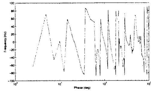
Figure 5-5: MIMO Controller Open Loop G_{yw} Transfer Functions
