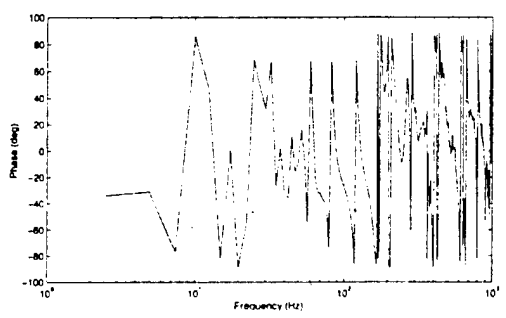
G_{y1u2} : PZT2-to-Mic1
