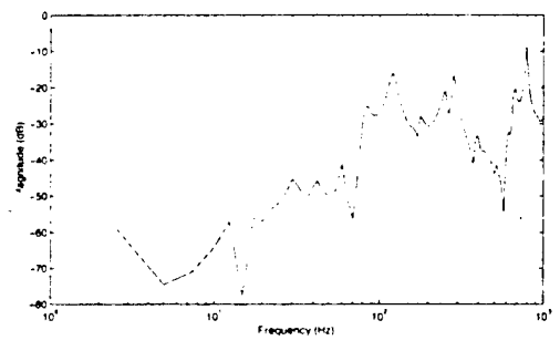
G_{y1u2} : PZT2-to-Mic1
