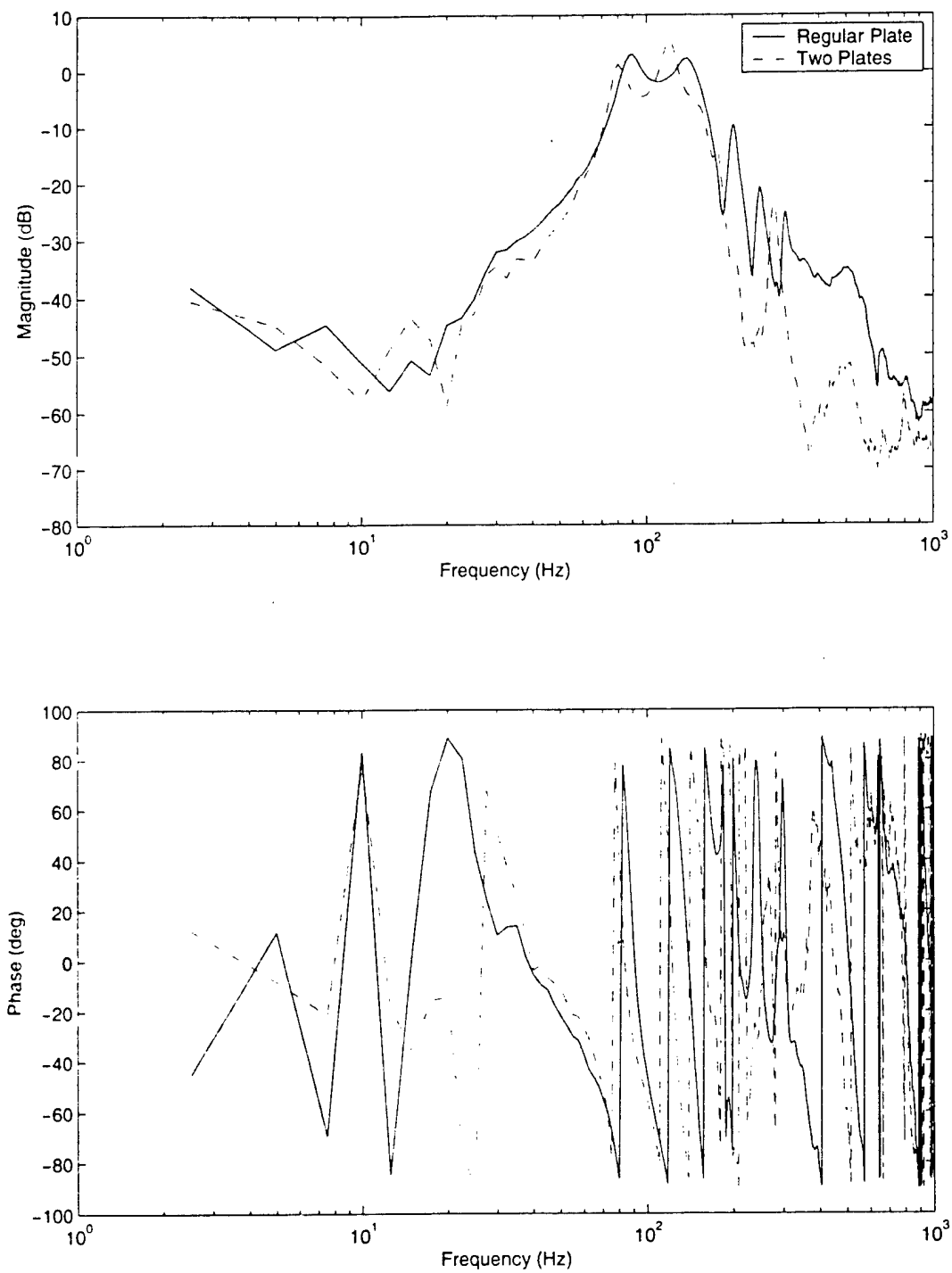
Figure 5-2: Regular Plate vs. Two Plates (9.875 in apart)
