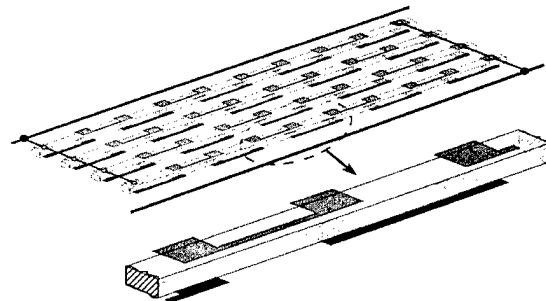
Figure 7. PZT dendrite with ribbon fibers with a 3:1 aspect ratio ( 600 \times 200 \mu - m ).
