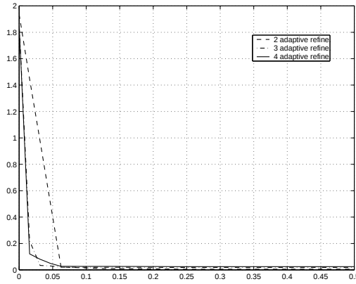
FIG. 7.4. Example solutions of the test problems low and low J respectively.
