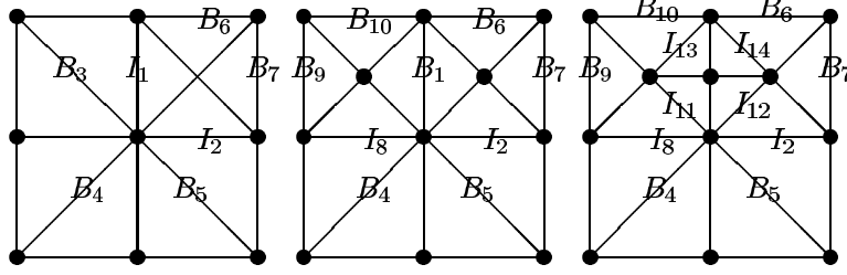
FIG. 6.5. The interface-base edges marked by I sit between two different levels of refinement. Once an interface-base edge has been updated to a base edge, it may be bisected.
