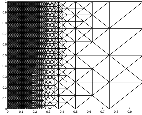
FIG. 6.7. Example grid at time step 20, contains 4390 nodes.
