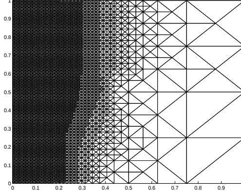
FIG. 6.8. Example grid at time step 30, contains 5602 nodes.
