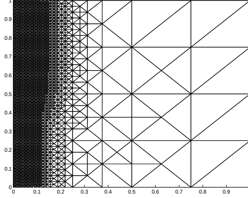
FIG. 6.6. Example grid at time step 10, contains 2868 nodes.
