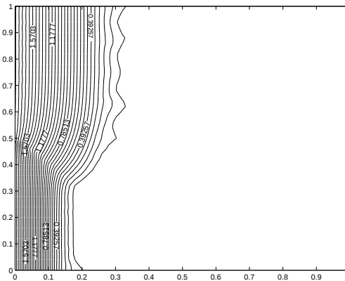
FIG. 7.5. Example solution at time step 32 with \alpha = -2 .
