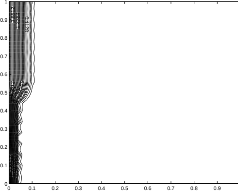
FIG. 7.7. Example solution at time step 32 with \alpha = -3 .
