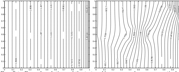
FIG. 7.1. Example solutions of the test problems low and low J respectively.
