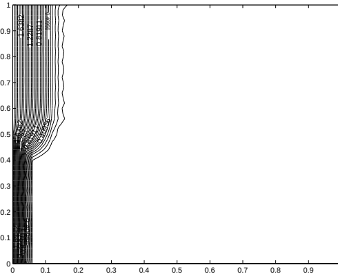
FIG. 7.8. Example solution at time step 64 with \alpha = -3 .
