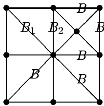
In terms of the node-edge data structure, it is easier to work with the base edges rather than the newest nodes, where the base edges are the edges that sit opposite the newest nodes, such as those marked by B in Figure 6.1.
