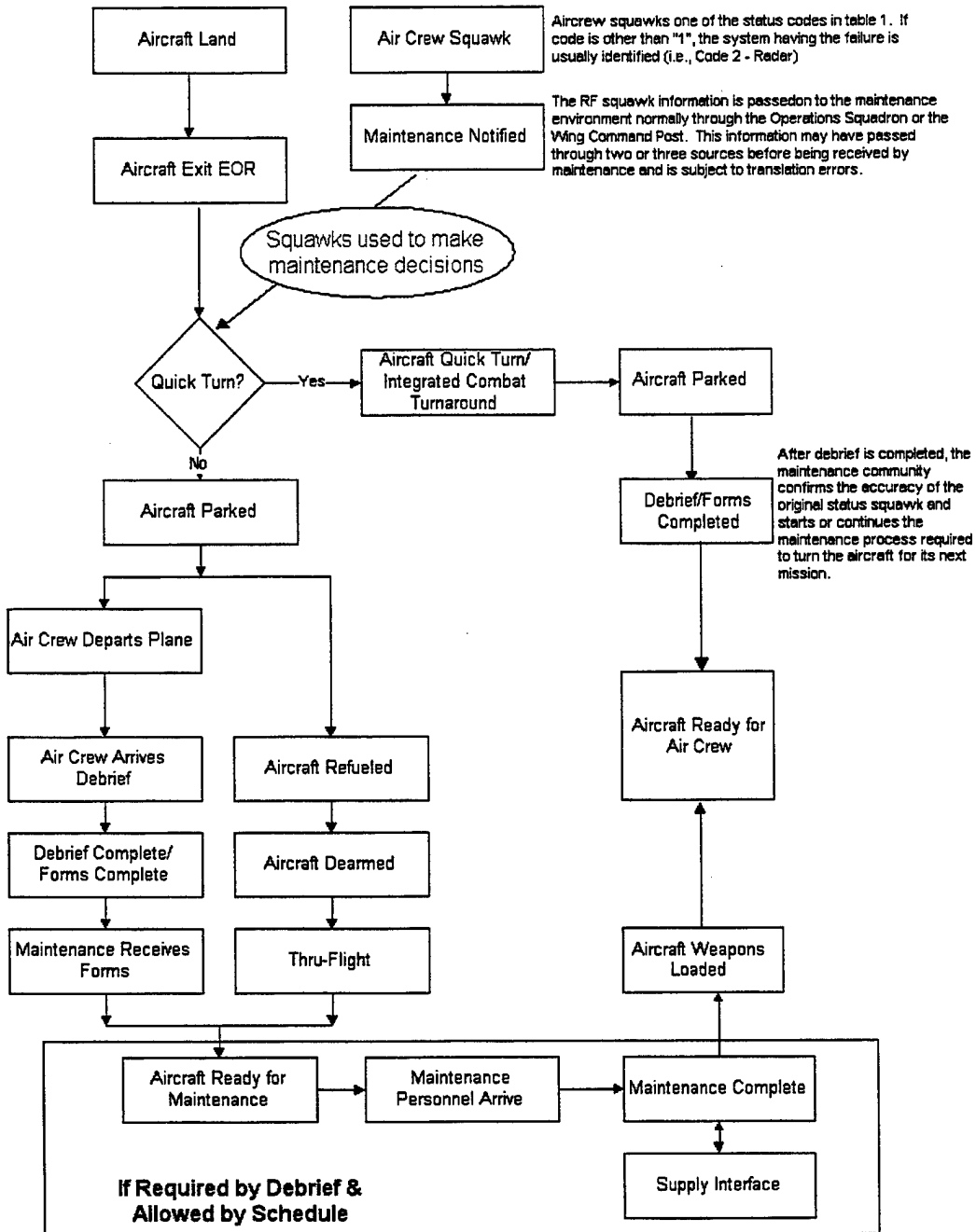
Figure 2 – AS-IS Aircraft Maintenance Flow
