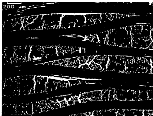
C/C specimen after pyrolysis up to 900 °C (fibre pretreatment temperature 600 °C, fluorescensc optical microscopy)
