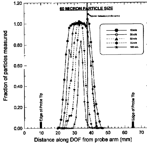
Figure 3. Measured response of a 2DC probe, as a function of velocity, to a constant stream of 60\ \mu\text{m} particles across the entire length of the exposed laser. Plotted is a fraction of particles measured as a function of distance from the inside position of the laser side probe arm. The zero area images (ZAI) are included.
