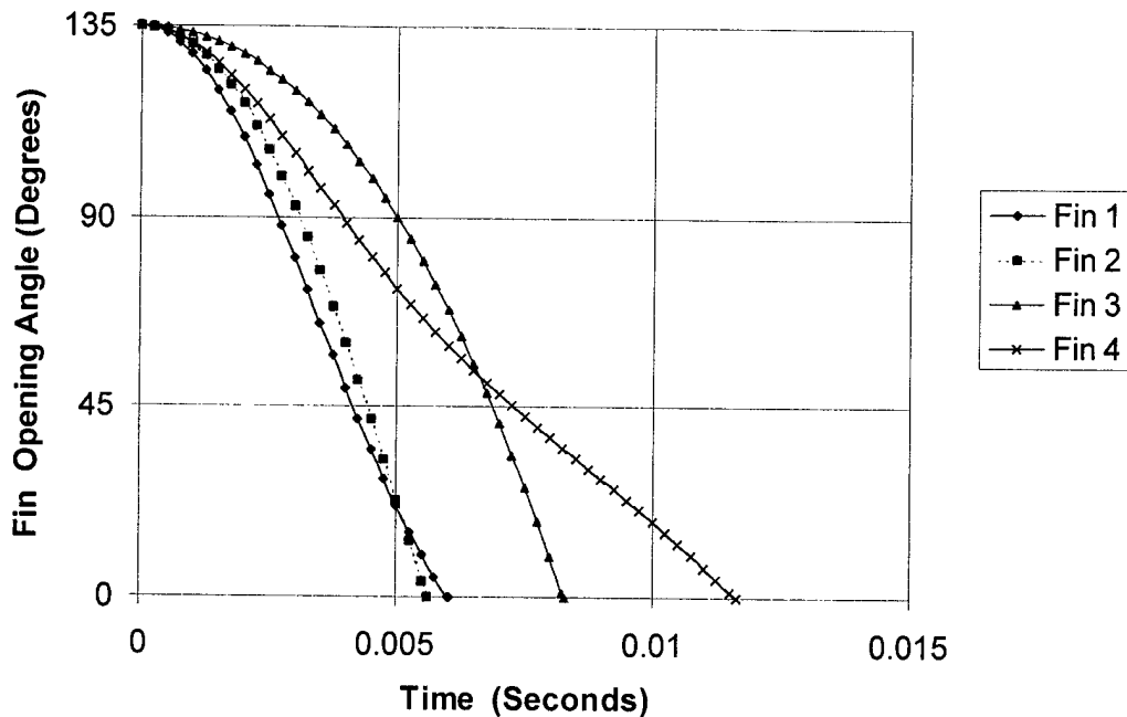
Figure 13. Fin Opening Angle as a Function of Time, 5 degrees of Yaw, 30-Hz Spin Rate.
