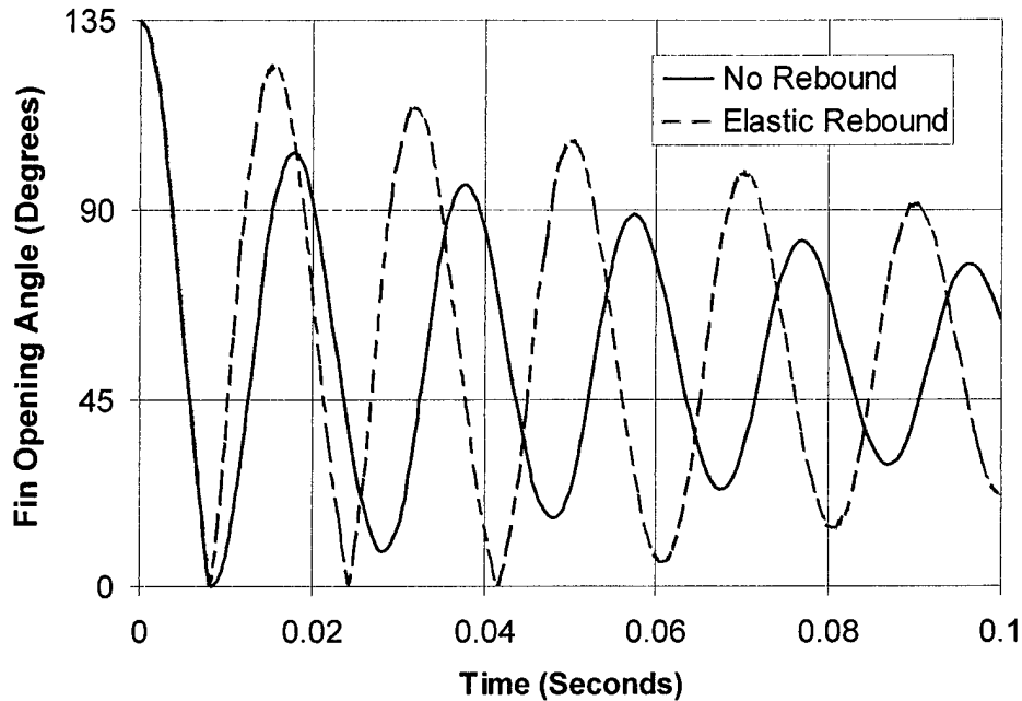
Figure 14. Fin Opening Angle as a Function of Time, No Locking Mechanism, Zero Yaw, 15.6-Hz Spin Rate.
