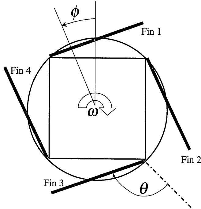
Figure 3. Schematic of Fin Opening.
