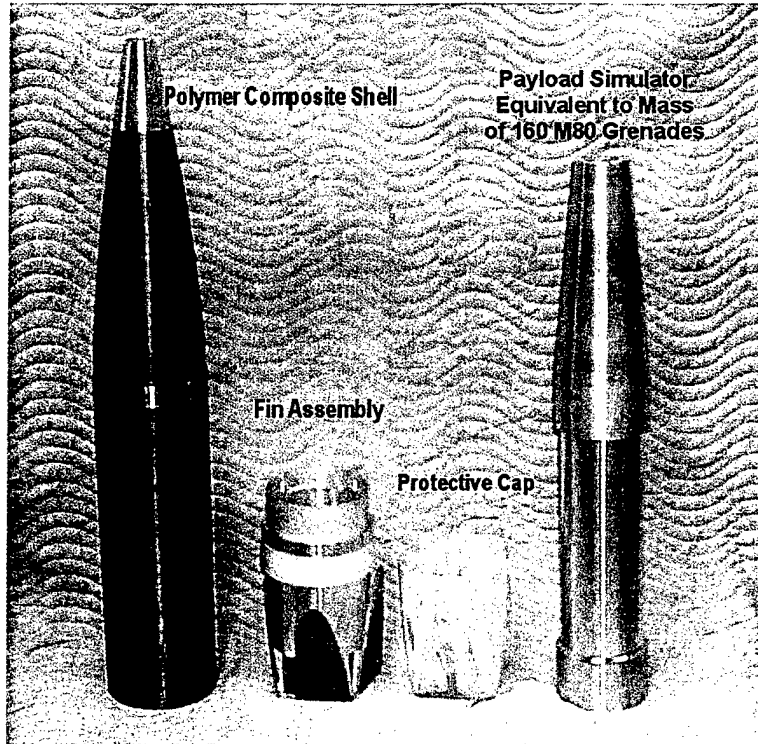
Figure 2. Components of a 75-pound Projectile.
