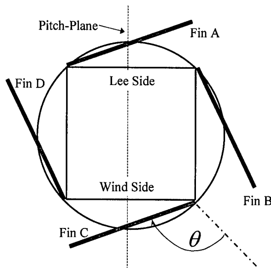
Figure 7. Schematic Showing Orientation of Fins A Through D Relative to Pitch Plane.
