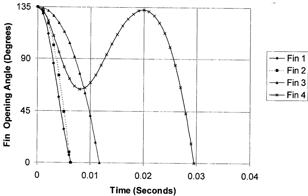
Figure 12. Fin Opening Angle as a Function of Time, 5 Degrees of Yaw, 15.6-Hz Spin Rate.
