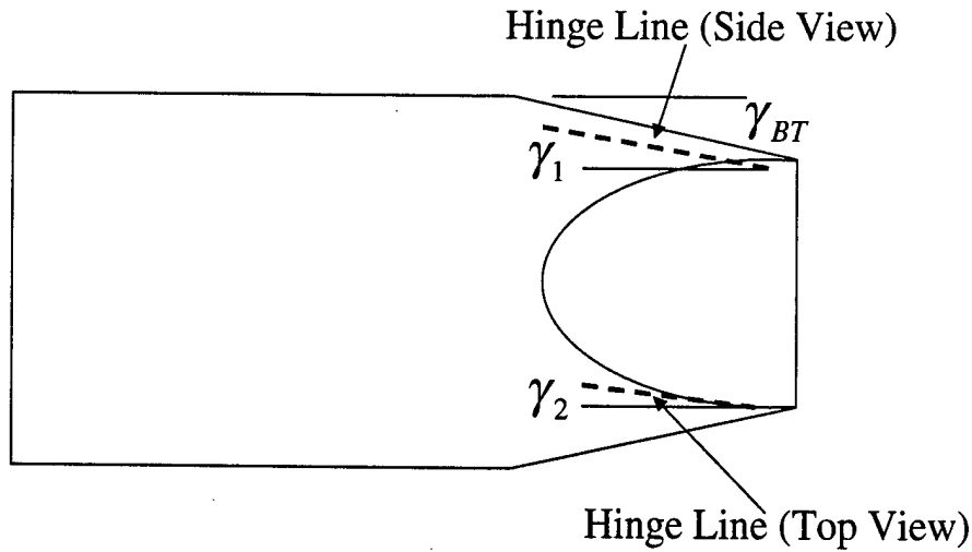
Figure 4. View of the Compound Angle of the Hinge Line.
