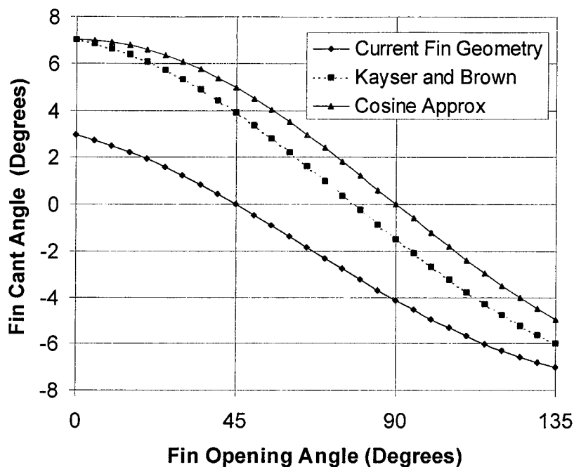
Figure 5. Effective Fin Cant Angle as a Function of Fin Opening Angle.
