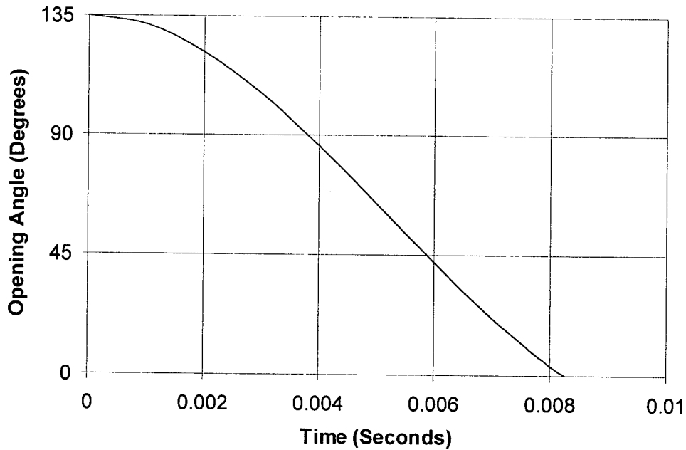
Figure 11. Fin Opening Angle as a Function of Time, Zero Yaw, 15.6-Hz Spin Rate.
