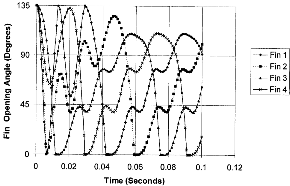
Figure 15. Fin Opening Angle as a Function of Time, No Locking Mechanism, 5 Degrees of Yaw, 15.6-Hz Spin Rate.
