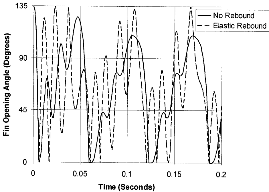
Figure 16. Fin Angle Response to Impact With Fin Stop as a Function of Time for No Locking Mechanism, 5 Degrees of Yaw, 15.6-Hz Spin Rate.
