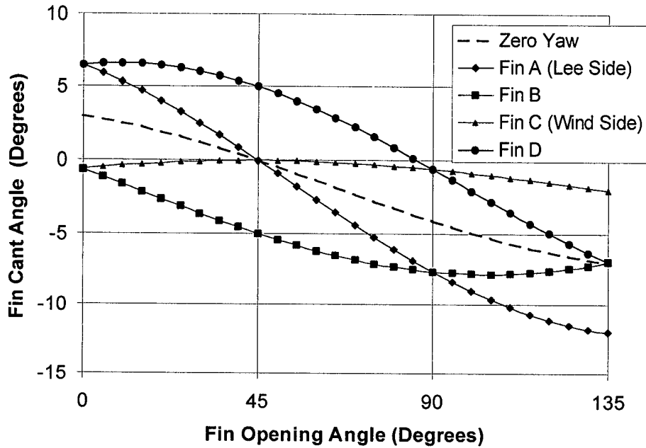
Figure 6. Effective Fin Cant Angle as a Function of Fin Opening Angle, Zero Yaw and Zero Spin.
