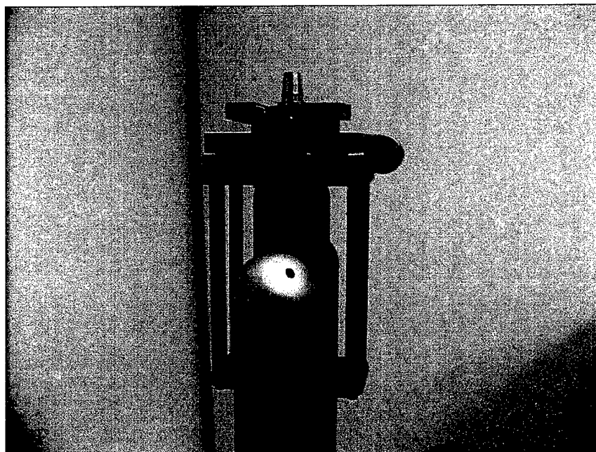
Figure 18. Inlet calibration device assembly installed on SPEC FSSP-100.
