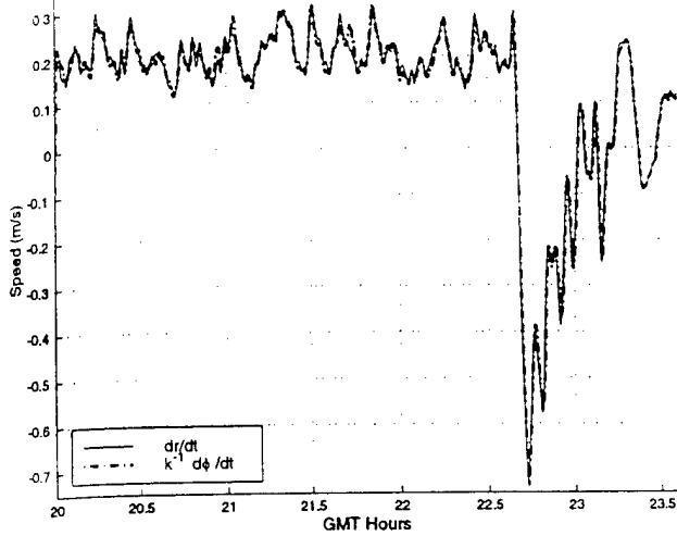
Fig. 4. Comparison of GPS-derived phase rate (solid line) with phase model results (dashed line) obtained using MOMAX I - 50 Hz data.
