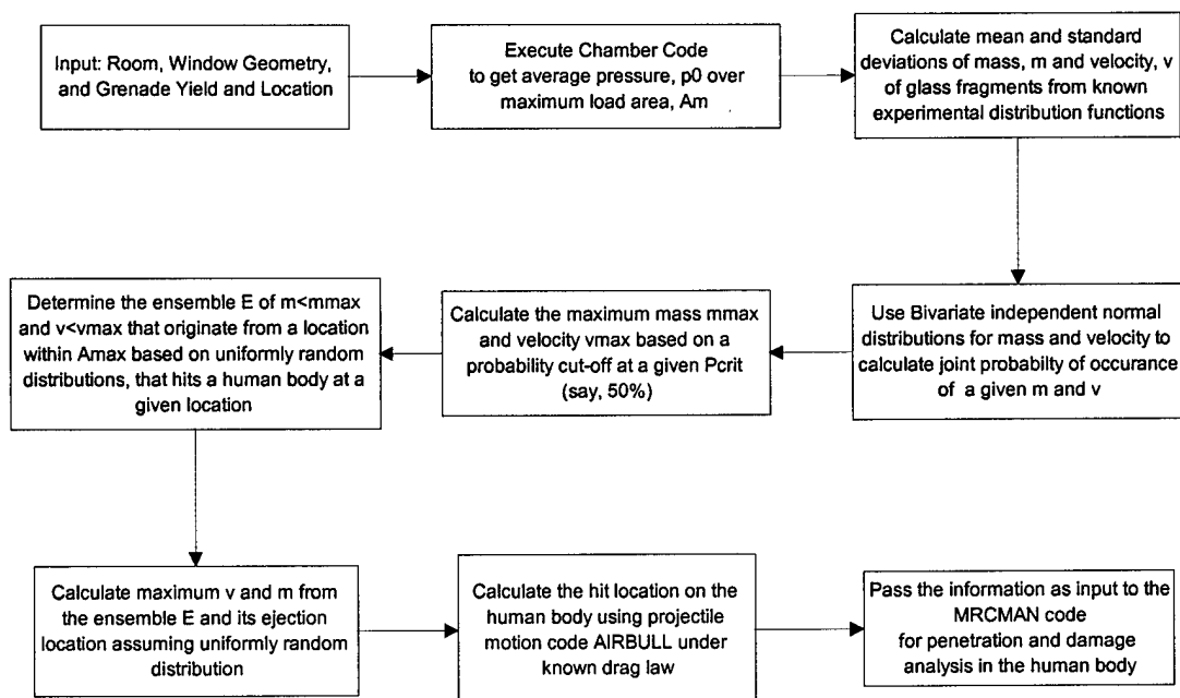
Figure 3. Flow-Chart of how "Worst Case" Fragment is used in Conjunction with MRCMAN Character Simulator.
