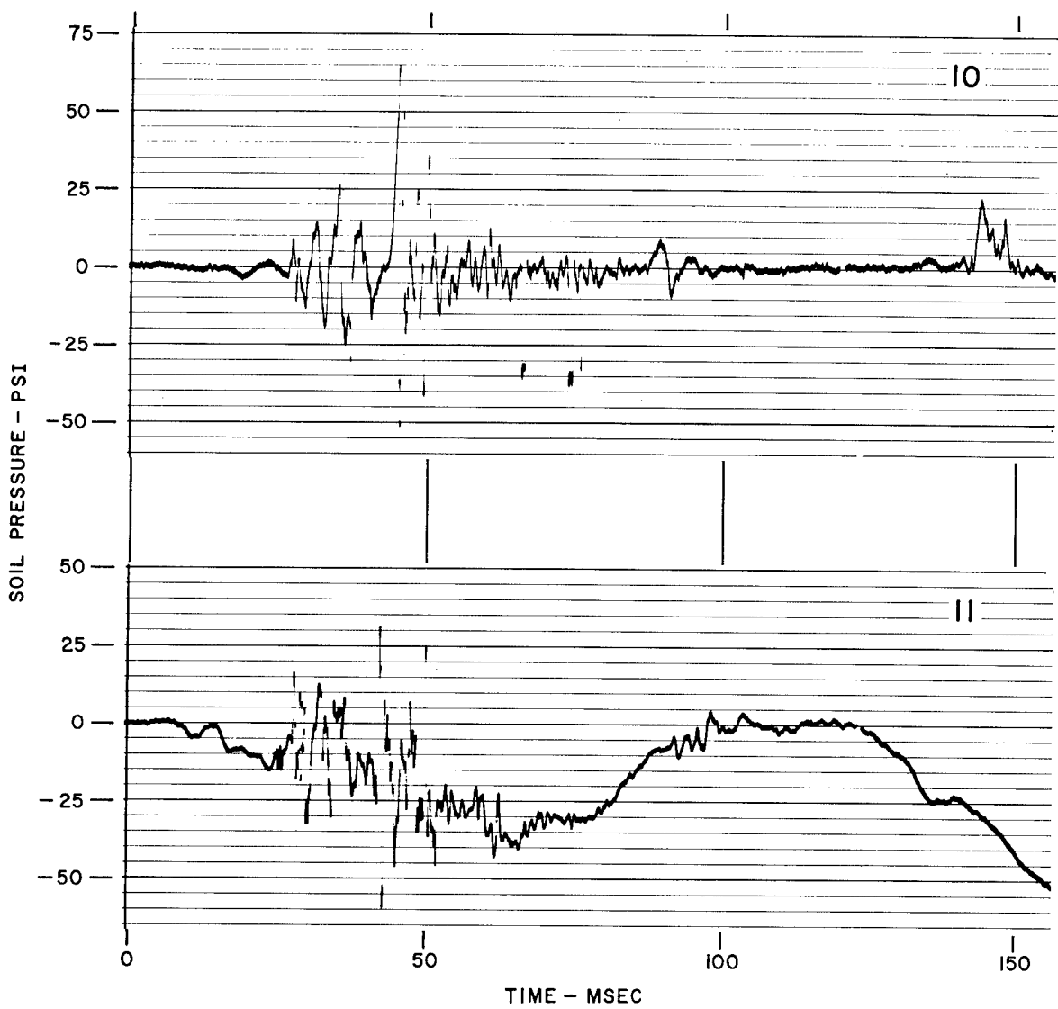
Figure 3.20. --Soil pressures on air-shaft wall, PRAIRIE FLAT Event.
