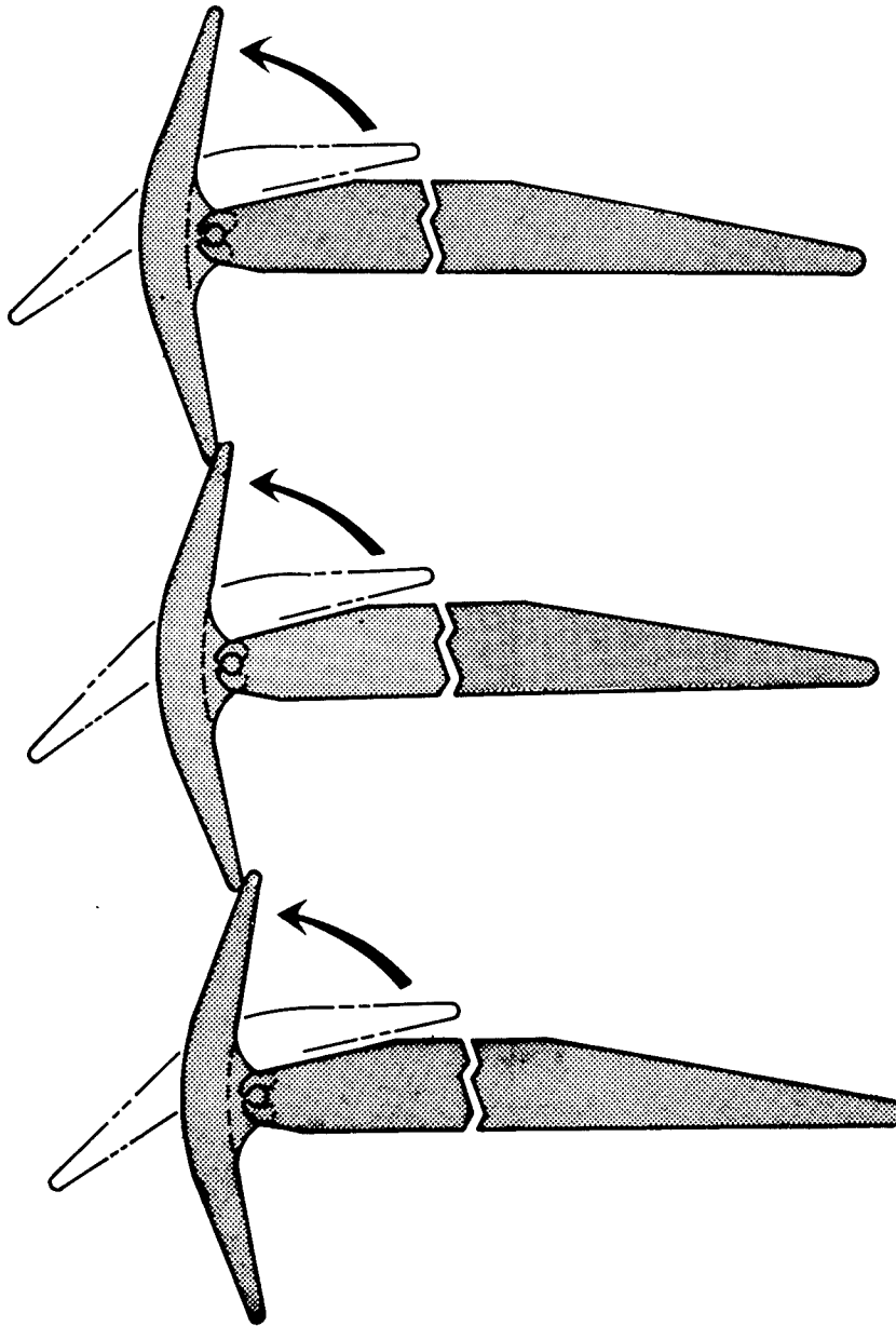
Figure 1.4. --Louver operation.
