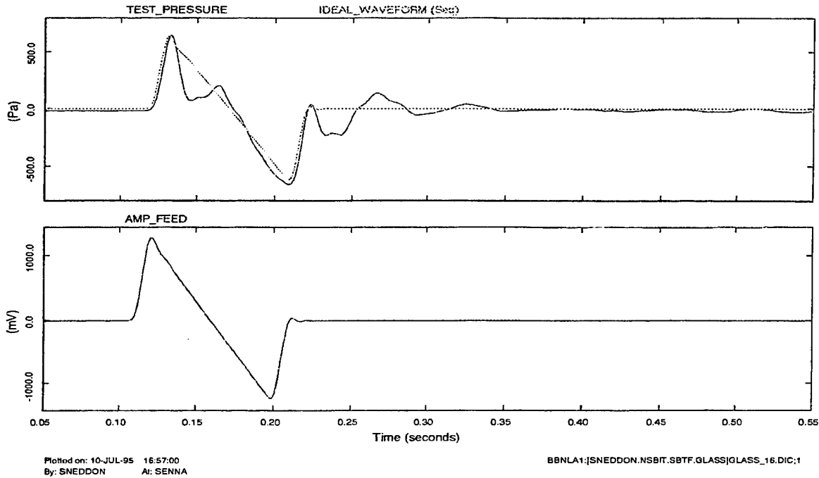
Figure 2-11. Typical SBTF Uncompensated Sonic Boom Waveform.
