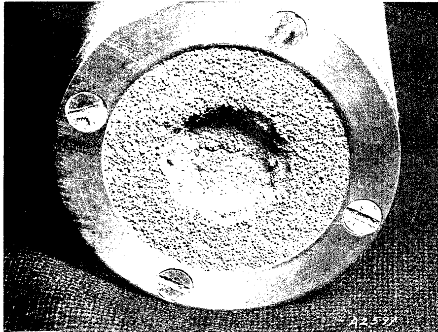
Front view showing filter (porous bronze) disk which was forced back into diaphragm cavity on 2000 psi transducer piezometer by force of blast from SC-2
