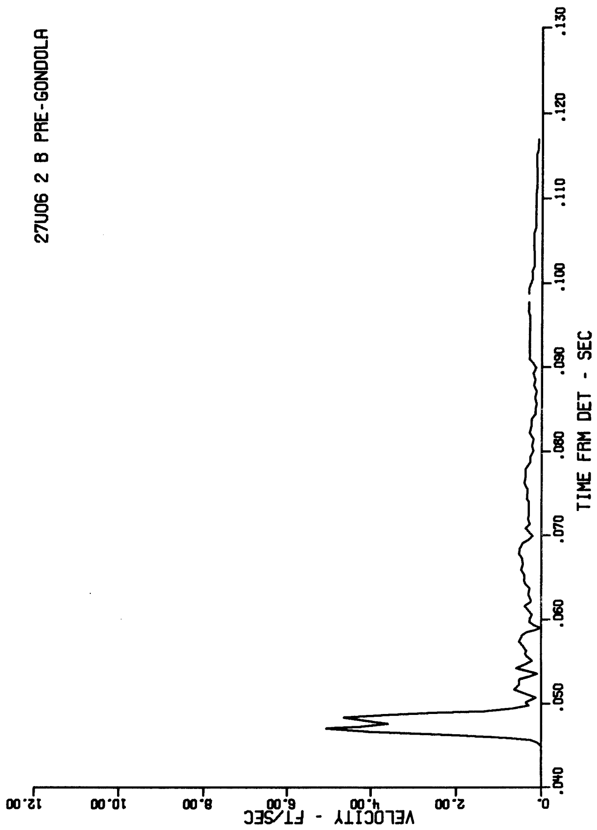
Figure A.18 Gage 27-u-6, range 300 ft, depth 46 ft, Event Bravo
