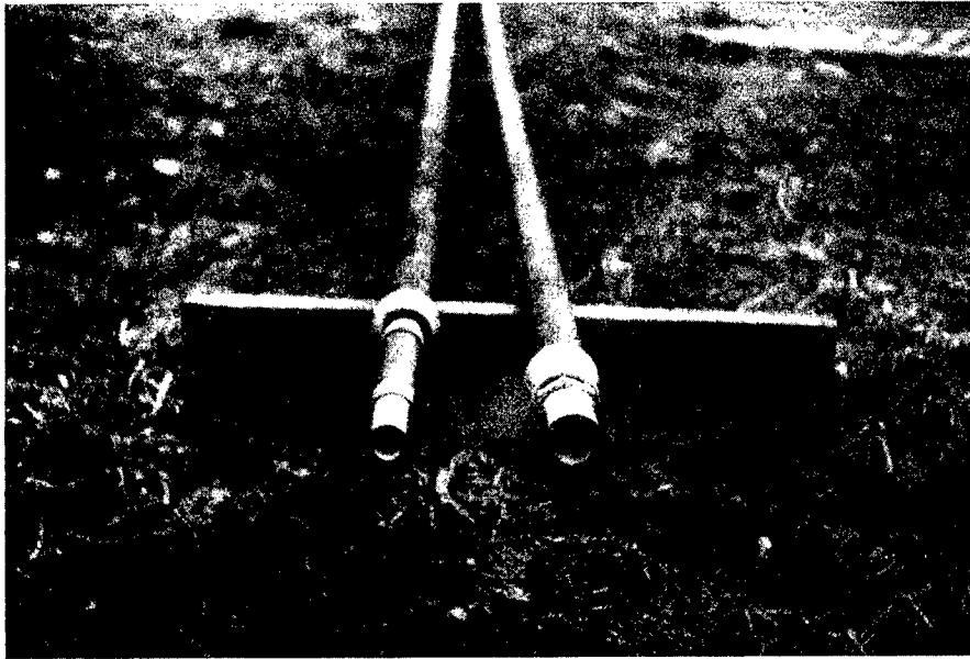
a. UA piezometer (left) and WES transducer piezometer (right) before filter disks were attached
