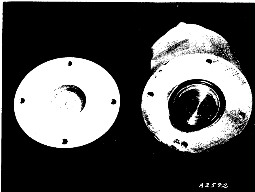
b. End view of piezometer with filter ring removed. Note diaphragm end of transducer fits into cavity on back side of filter ring
