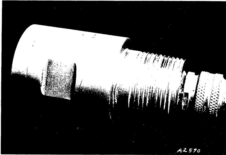
a. Side view of piezometer housing for WES-built CEC transducer piezometer (OD = \pm 1\text{-}3/4 in.)
