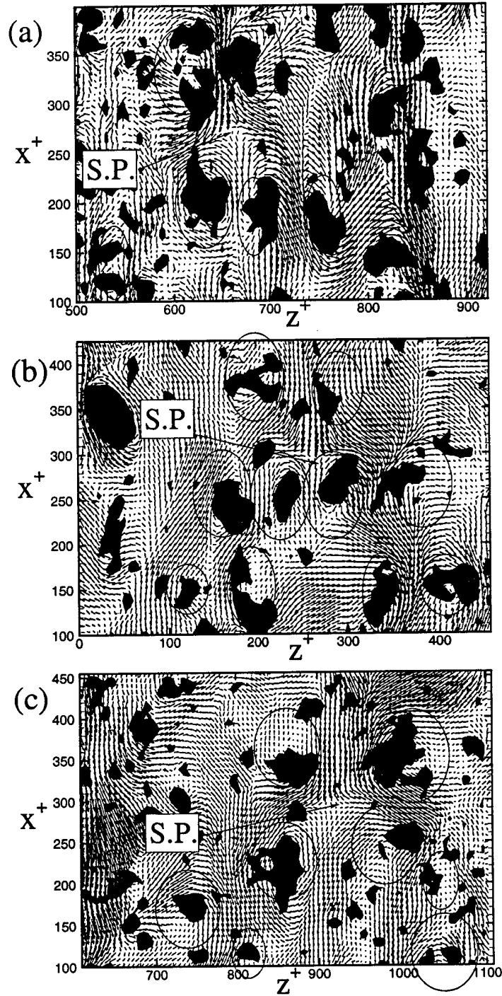
Figure 2. Evidence for scale growth via vortex leg annihilation and packet merging. Instantaneous vector fields are shown with contours of swirling strength multiplied by the sign of vorticity at Re_\theta = 1015 . The plots reveal the “signature” of merging vortex packets: coalescing low-speed regions bordered by vortices upstream and downstream of the merge location. A stagnation point (“S.P.”) appears where the streaks combine. (a) y^+ = 21 ; (b) y^+ = 46 ; (c) y^+ = 92 .
