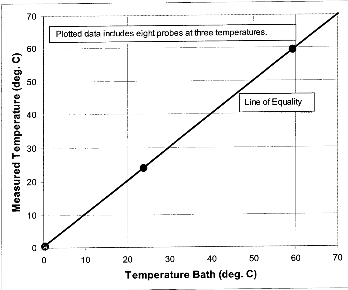
Figure 4. Verification data for Campbell scientific model 108 temperature probes [ F = (9/5) * (°C) + 32 ]
