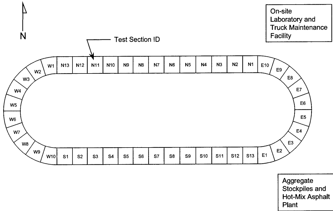
Figure 1. Track layout
