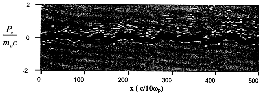
Figure 11. Momentum of electrons in plasma wave.
